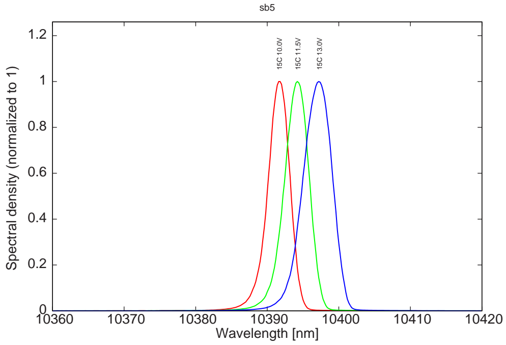
Figure 9: spectra at 15°C for various LDD voltages
