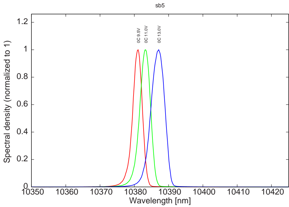
Figure 8: spectra at 0^{\circ}\text{C} for various LDD voltages
