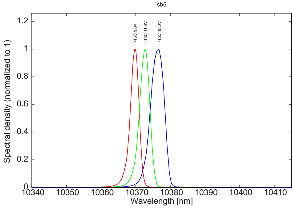
Figure 7: spectra at -15^{\circ}\text{C} for various LDD voltages
