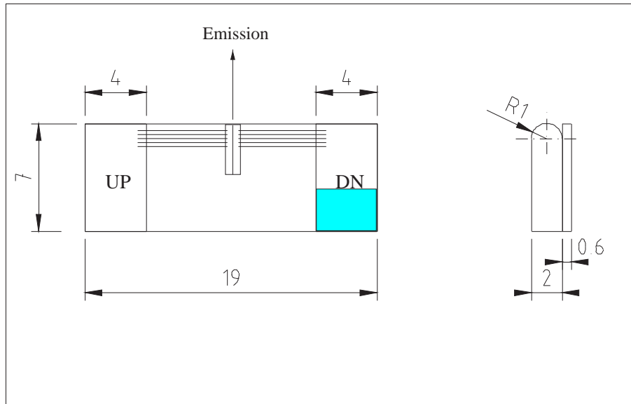
Figure 1: Support mounting for sb5 (please note that the laser is connected to the DN pad drawn in blue)
