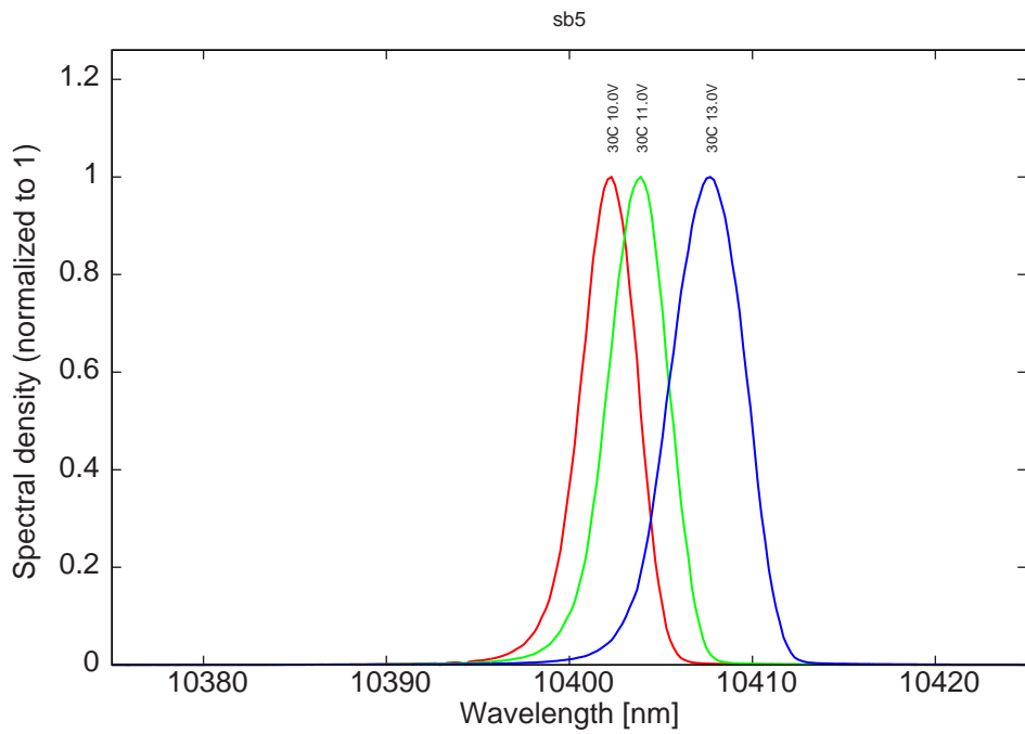
Figure 10: spectra at 30°C for various LDD voltages
