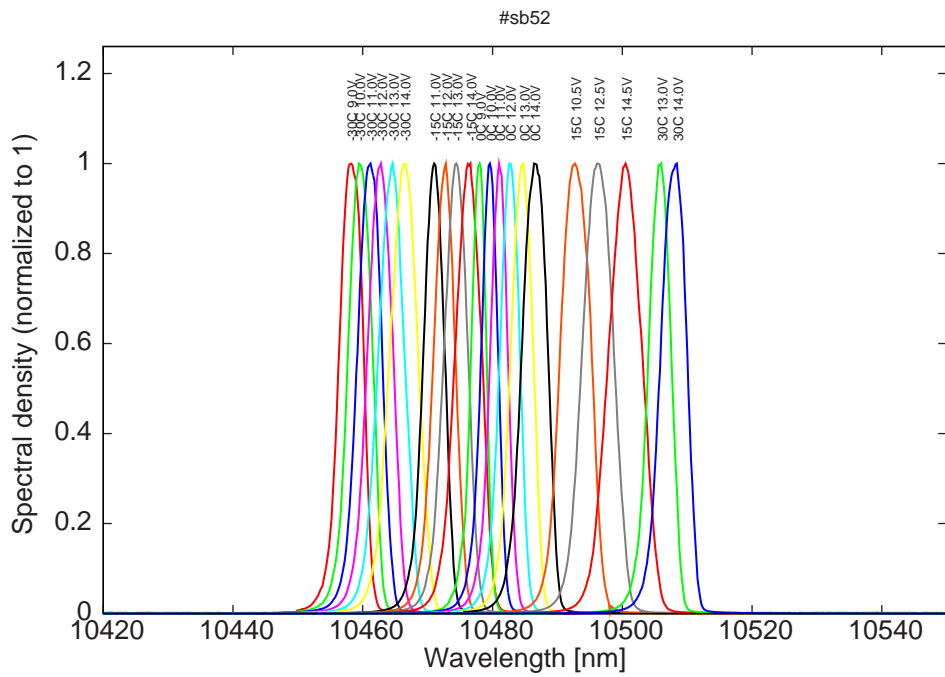
Figure 6: spectra for various temperatures and LDD voltages
