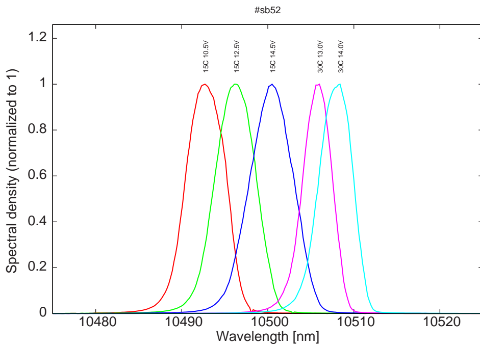
Figure 10: spectra at 15C and 30C for various LDD voltages
