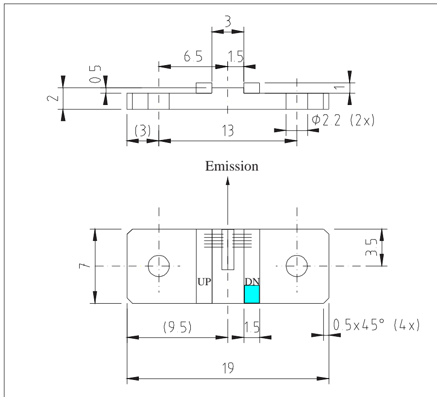
Figure 1: Support mounting for #sb525 DN (please note that the laser is connected to the DN pad drawn in blue)
