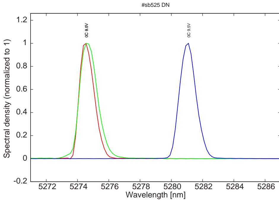
Figure 9: spectra at 0C for various LDD voltages ( mode jumping at 0C and 9.5V)
