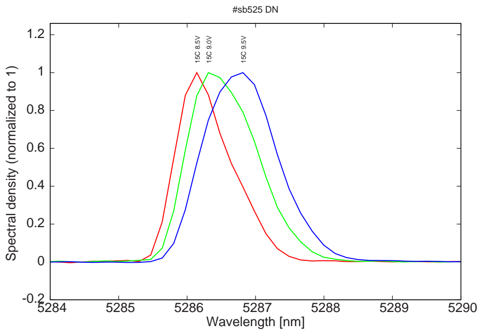
Figure 10: spectra at 15C for various LDD voltages (same mode as 0C and 9.5V)
