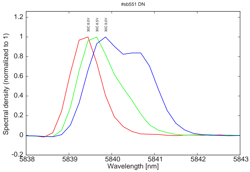
Figure 11: spectra at 30C for various LDD voltages (holes in the spectra due to absorption in the air)
