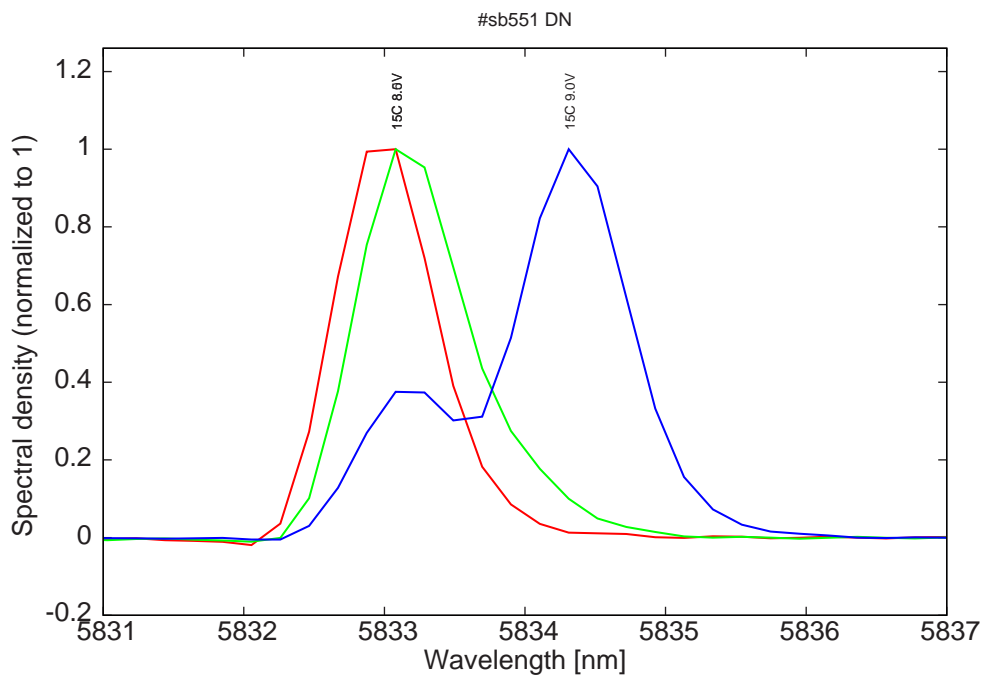
Figure 10: spectra at 15C for various LDD voltages (holes in the spectra due to absorption in the air)
