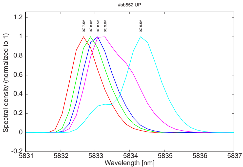
Figure 9: spectra at 0C for various LDD voltages (non-symmetric spectra due to absorption in the air)
