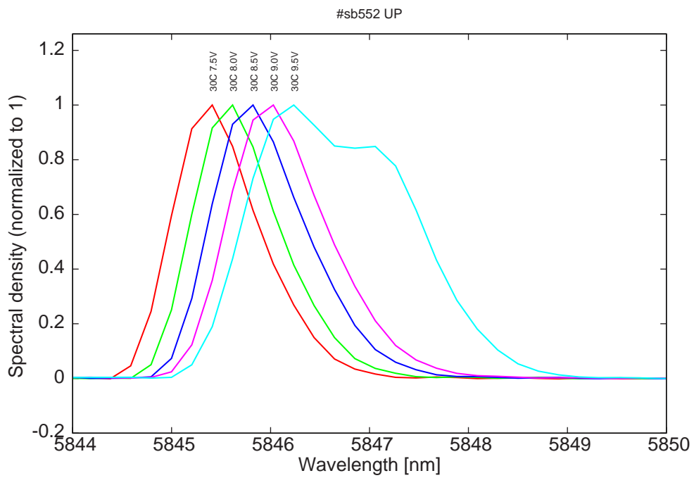
Figure 11: spectra at 30C for various LDD voltages (non-symmetric spectra due to absorption in the air)
