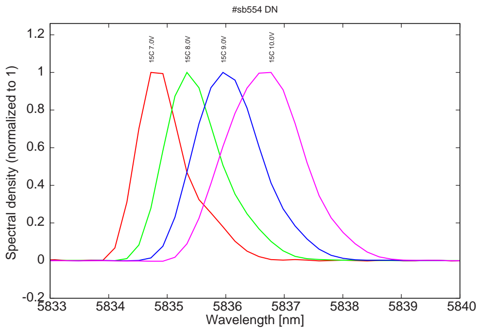
Figure 12: spectra at 15C for various LDD voltages
