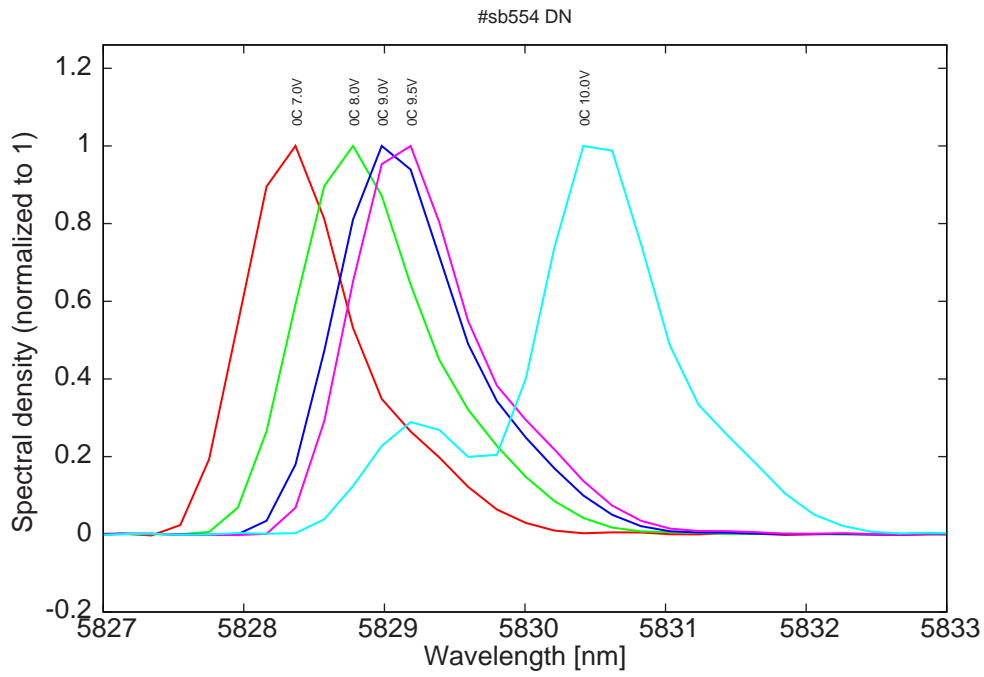
Figure 11: spectra at 0C for various LDD voltages (hole in spectrum at 10V due to absorption in the air)
