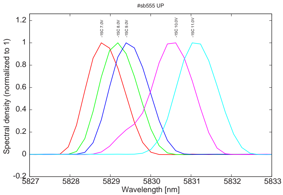
Figure 8: spectra at -15C for various LDD voltages (non-symmetric spectra due to absorption in the air)
