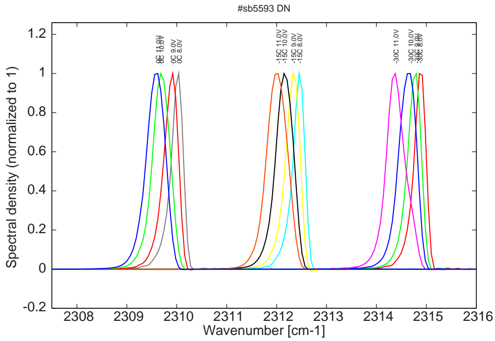
Figure 8: spectra between -30C and 0C for various LDD voltages (all monomode up to 11V on LDD)
