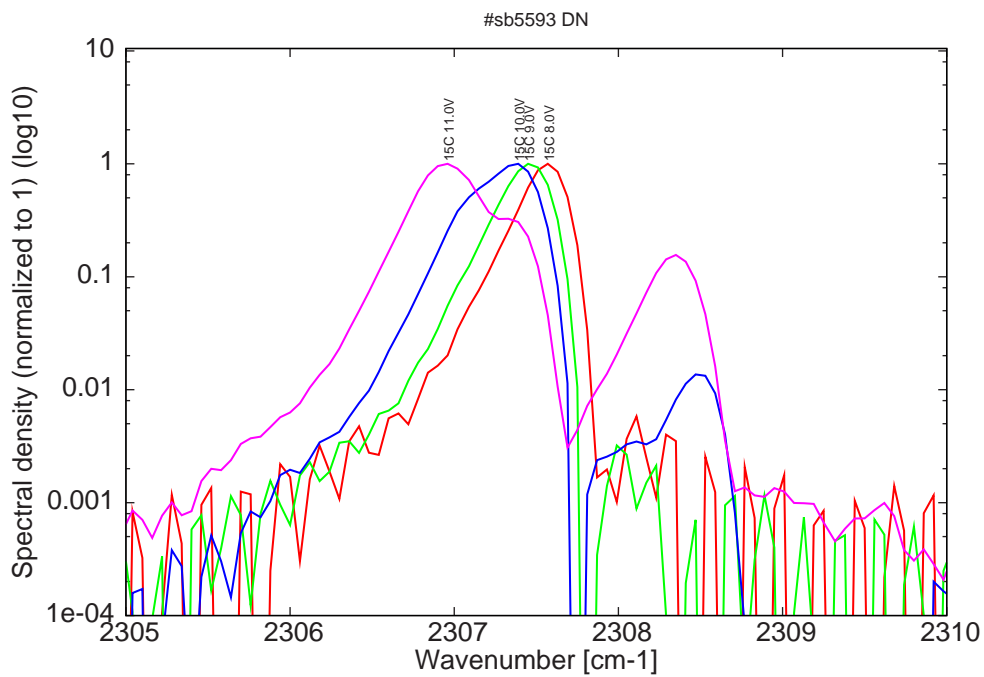
Figure 9: spectra 15C for various LDD voltages (become bimode at 10V on LDD)
