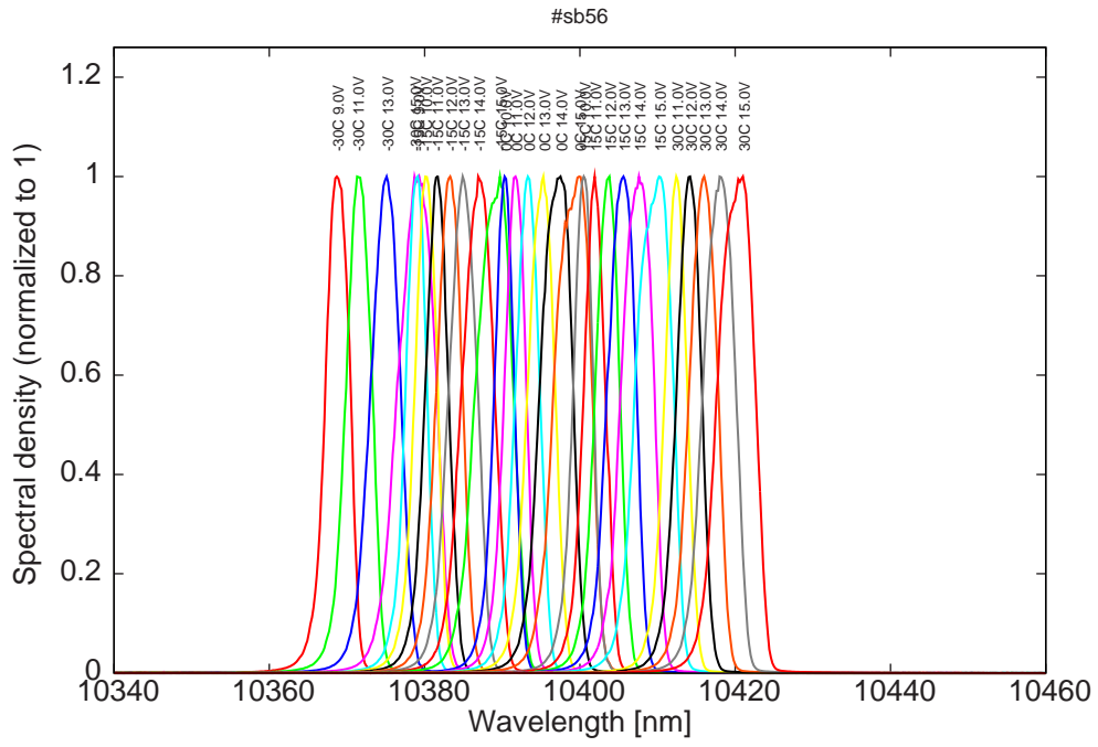
Figure 6: spectra for various temperatures and LDD voltages
