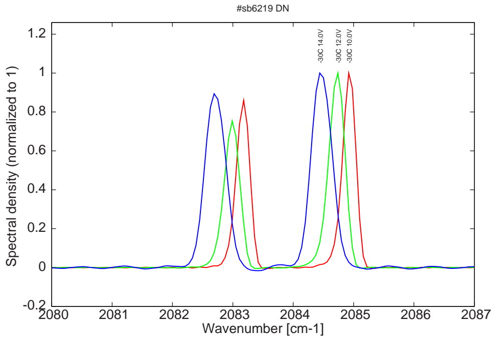
Figure 8: spectra at -30C for various LDD voltages (bimode)
