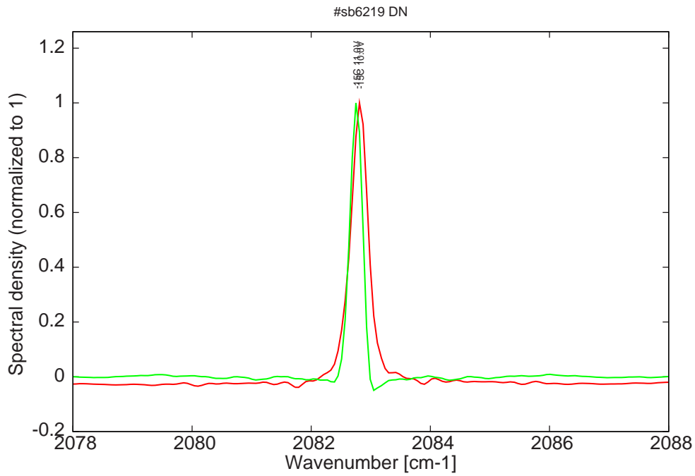
Figure 10: spectra at -15C for various LDD voltages (monomode range)
