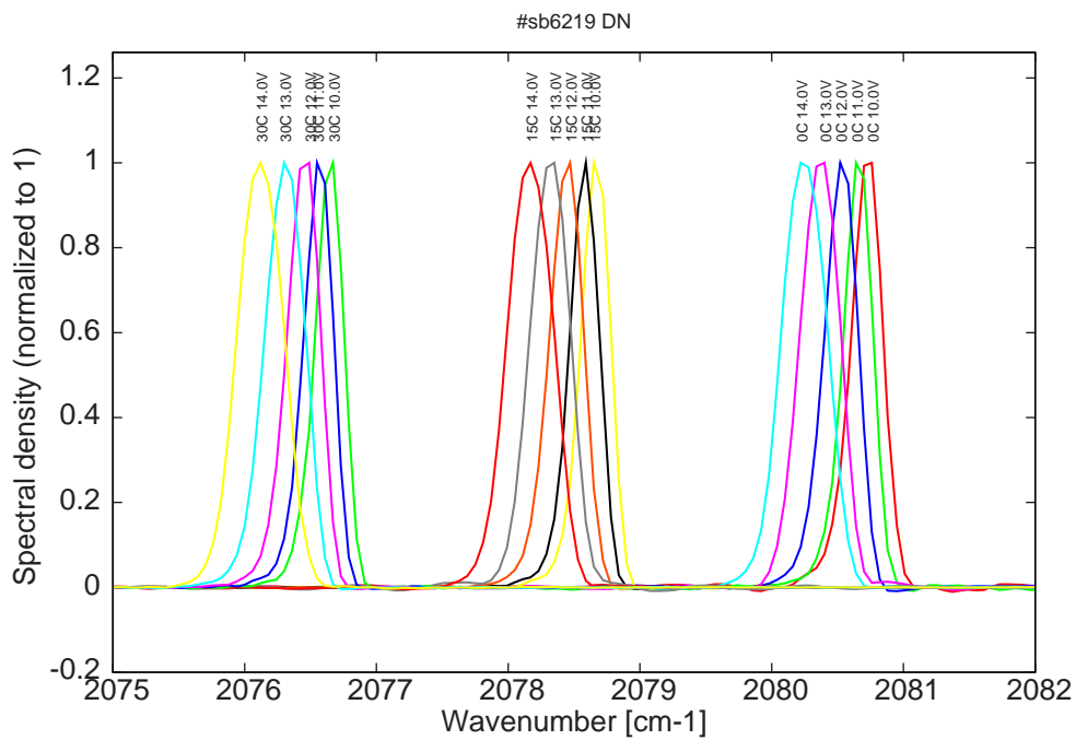
Figure 11: spectra between 0C and 30C for various LDD voltages (all monomode)
