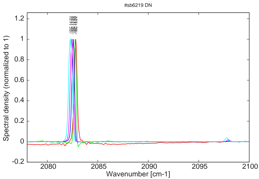
Figure 9: spectra at -15C for various LDD voltages (monomode up to 11V, then becomes bimode)
