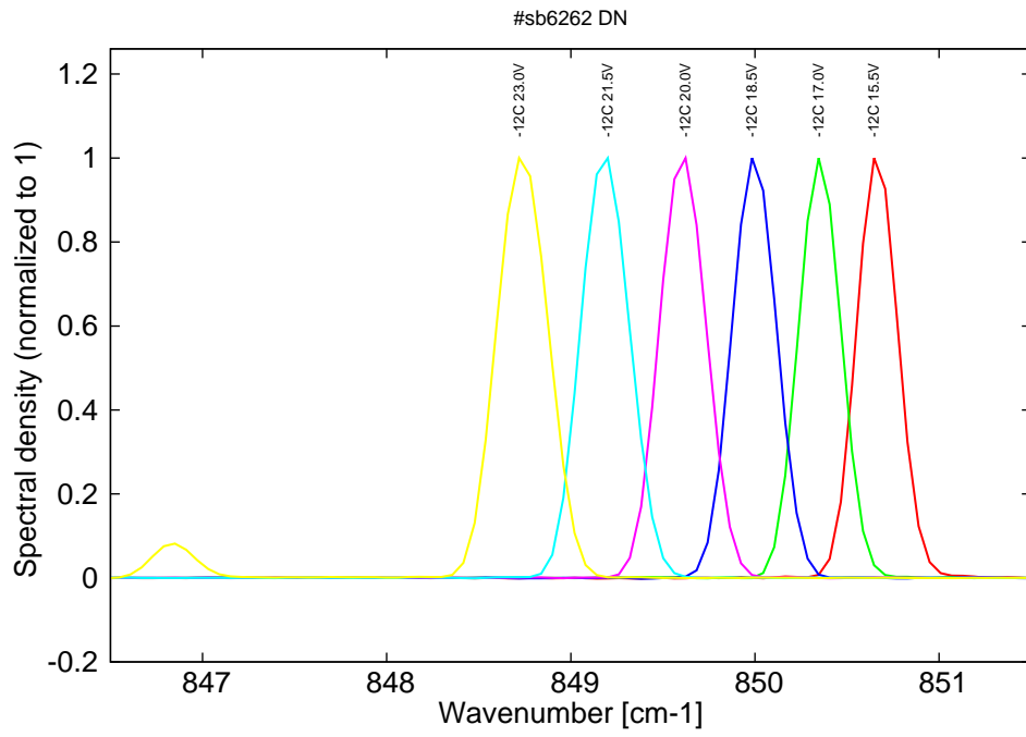
Figure 8: spectra at -12C at 3% duty-cycle (monomode up to 21.5V, then becomes bi-mode)
