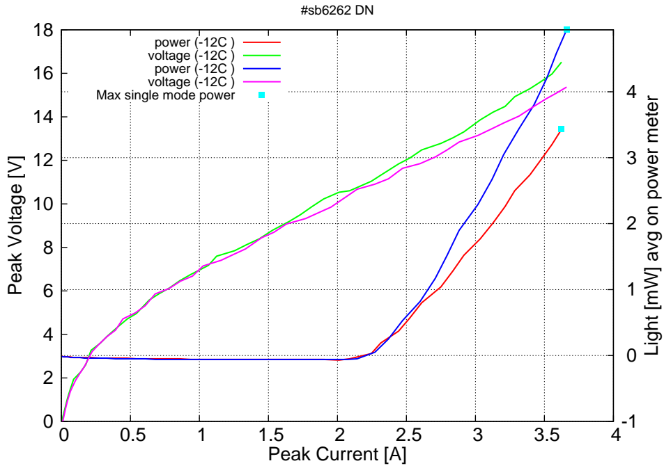
Figure 6: peak voltage and average power vs peak current at 2% (red) and 3% (blue) duty-cycle at -12C (50ns pulses on the laser) (the solid squares indicate the maximum singlemode emitted power)
