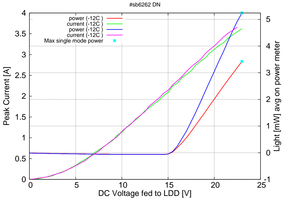
Figure 7: peak current and average power vs LDD voltage at 2% (red) and 3% (blue) duty-cycle at -12C (50ns pulses on the laser) (the solid squares indicate the maximum singlemode emitted power)
