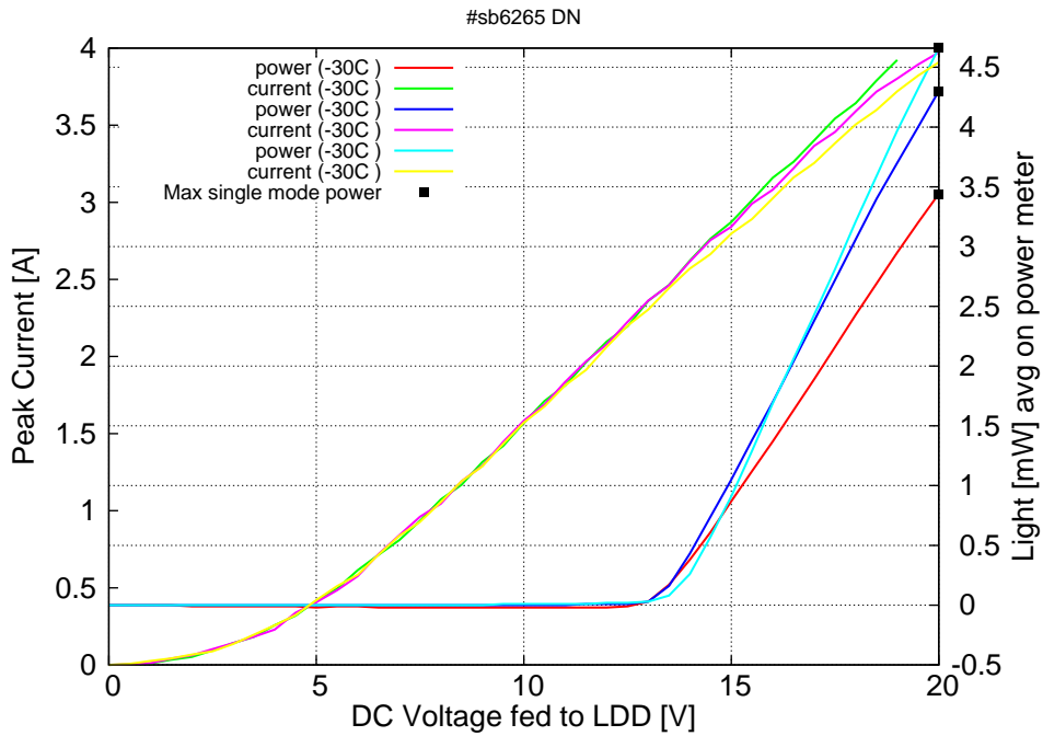
Figure 7: peak current and average power vs LDD voltage at 2% (red), 3% (blue) and 4% (cyan) duty-cycle at -30C (100ns pulses on the laser) (the solid squares indicate the maximum singlemode emitted power)
