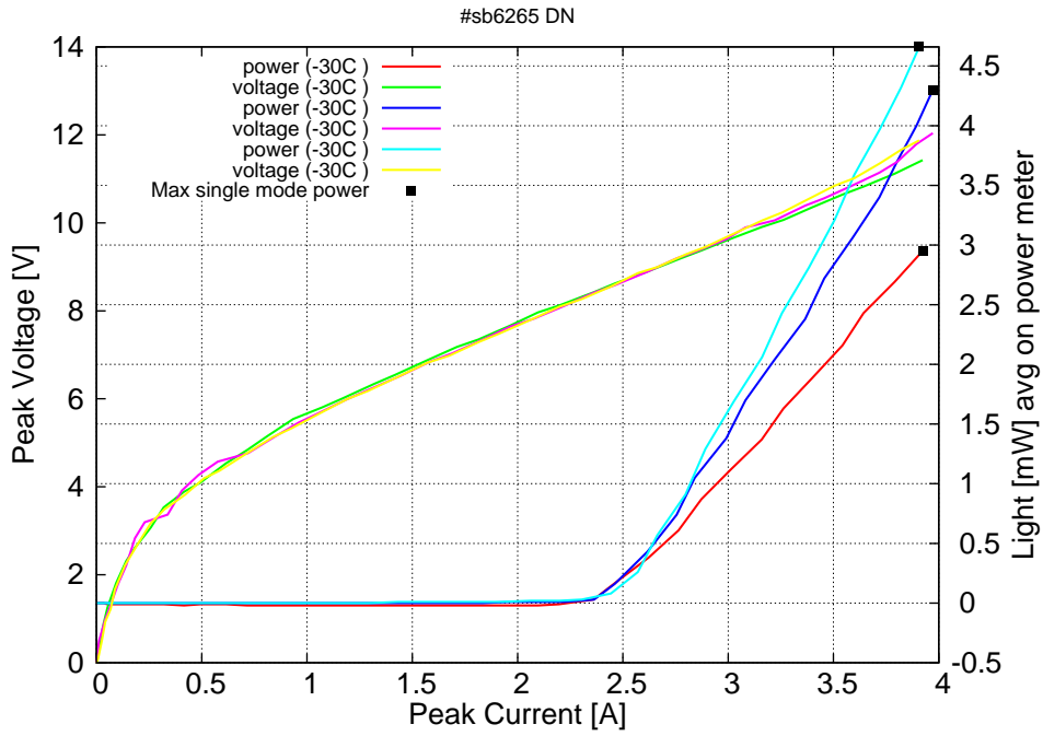
Figure 6: peak voltage and average power vs peak current at 2% (red), 3% (blue) and 4% (cyan) duty-cycle at -30C (100ns pulses on the laser) (the solid squares indicate the maximum singlemode emitted power)
