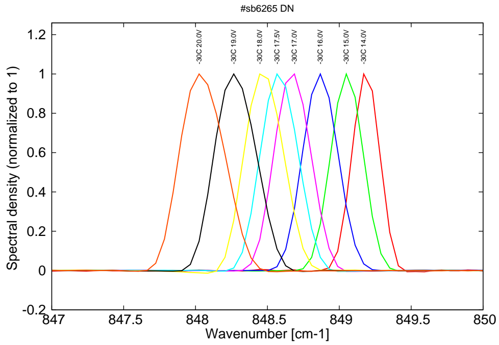
Figure 8: spectra at -30C at 4% duty-cycle
