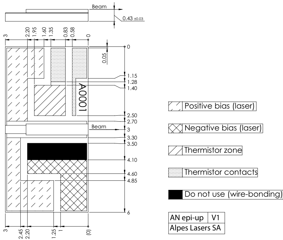
Figure 1: Mechanical and electrical interface for #sb6265 DN (please note that AlN submount numbering is 01614)
