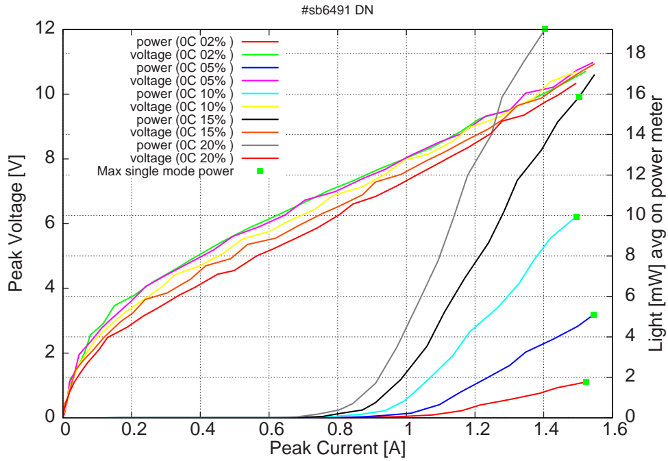
Figure 10: average power vs peak current at 0C for various duty-cycles (100ns pulses on the laser) (the solid squares indicate the maximum singlemode emitted power)
