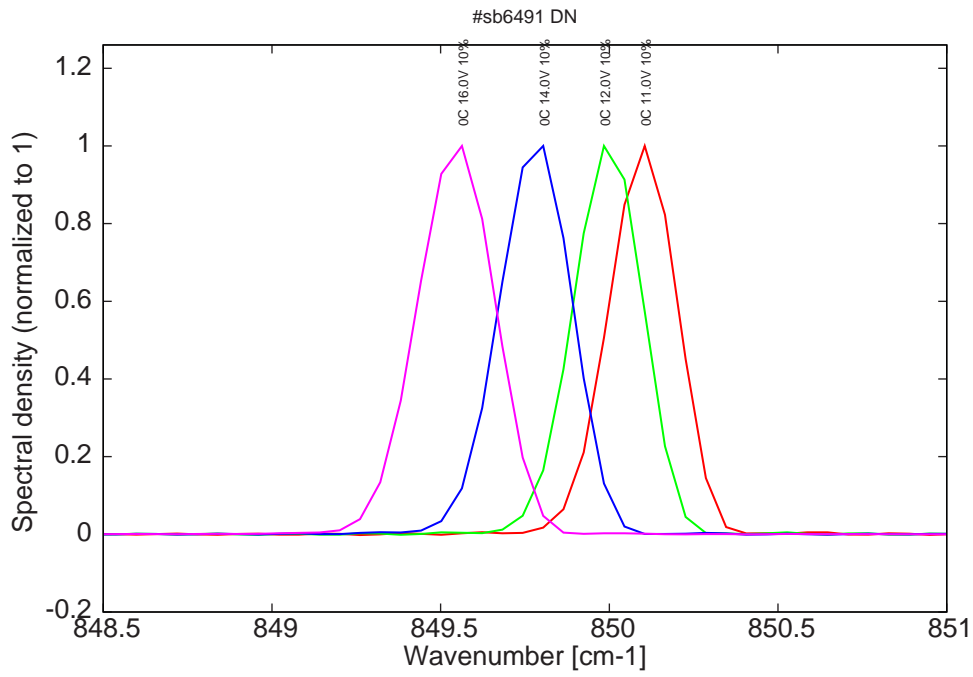
Figure 12: spectra at 0C at 10% duty-cycle (100ns pulses) for various LDD voltages (all monomode)
