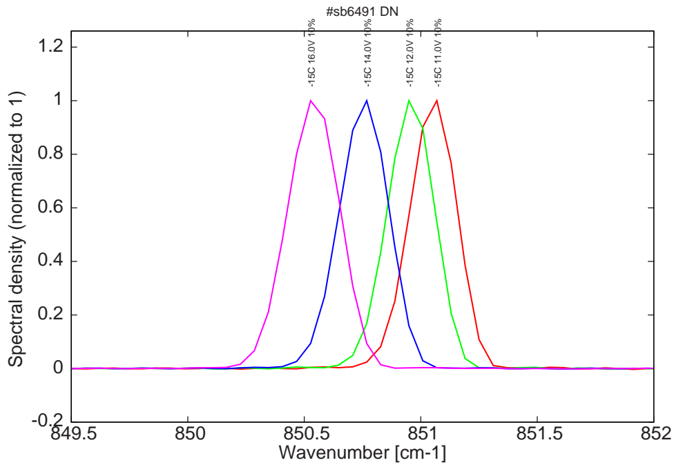
Figure 8: spectra at -15C at 10% duty-cycle (100ns pulses) for various LDD voltages (all monomode)
