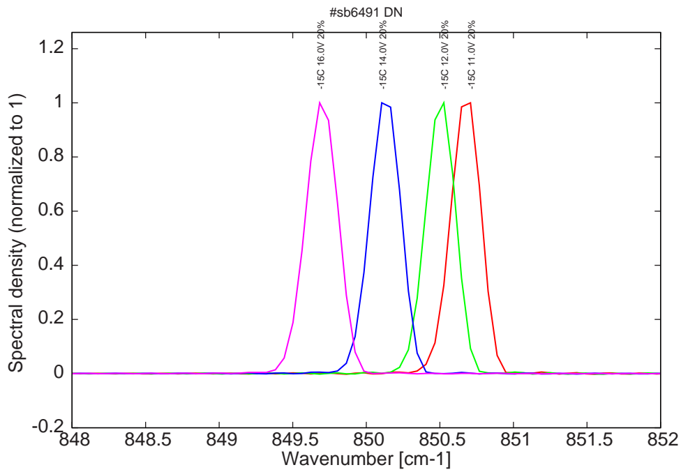
Figure 9: spectra at -15C at 20% duty-cycle (100ns pulses) for various LDD voltages (all monomode)
