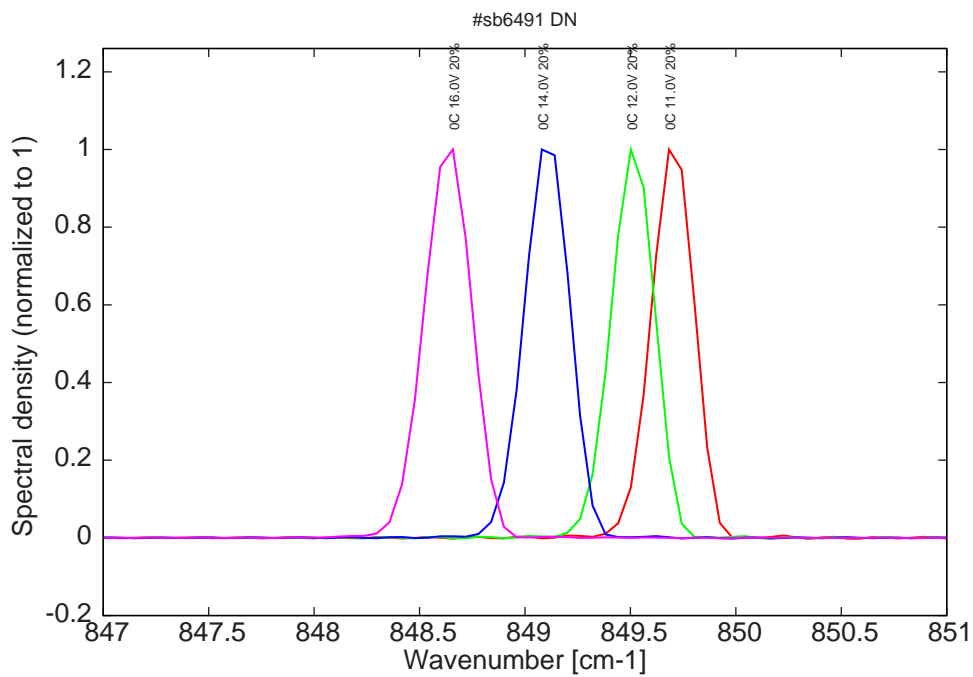
Figure 13: spectra at 0C at 20% duty-cycle (100ns pulses) for various LDD voltages (all monomode)
