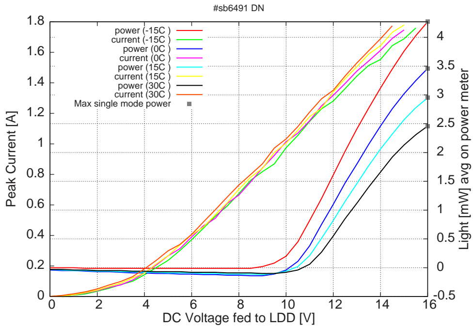
Figure 5: peak current and average power vs LDD voltage at 2% duty-cycle (50ns pulses on the laser) (the solid squares indicate the maximum singlemode emitted power)
