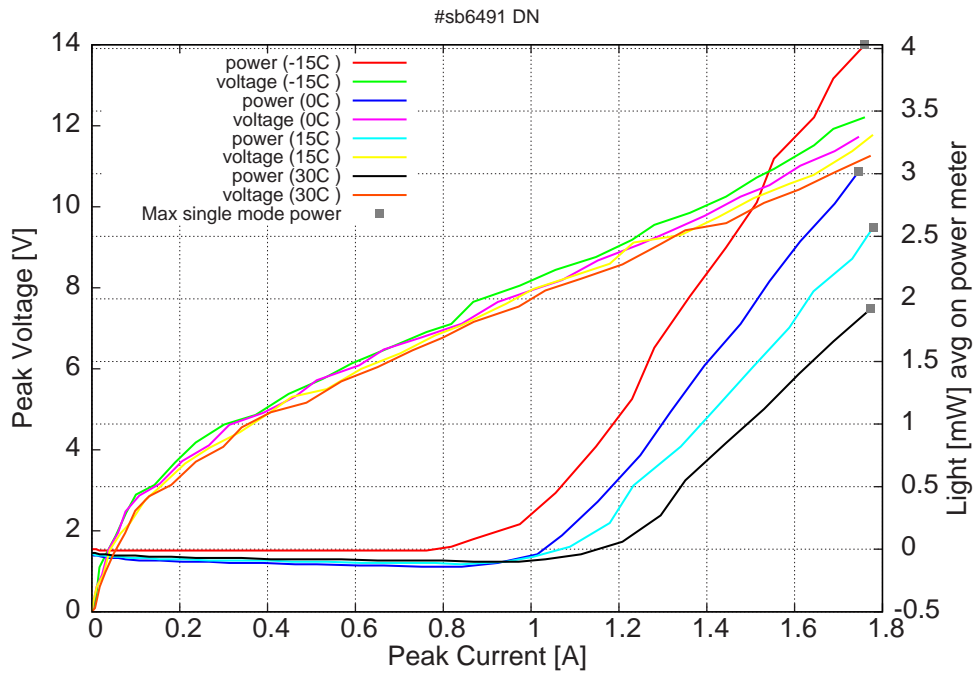
Figure 4: average power vs peak current at 2% duty-cycle (50ns pulses on the laser) (the solid squares indicate the maximum singlemode emitted power)
