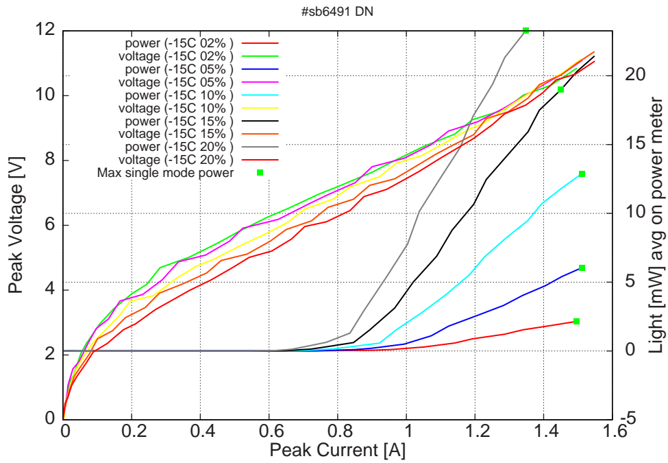
Figure 6: average power vs peak current at -15C for various duty-cycles (100ns pulses on the laser) (the solid squares indicate the maximum singlemode emitted power)
