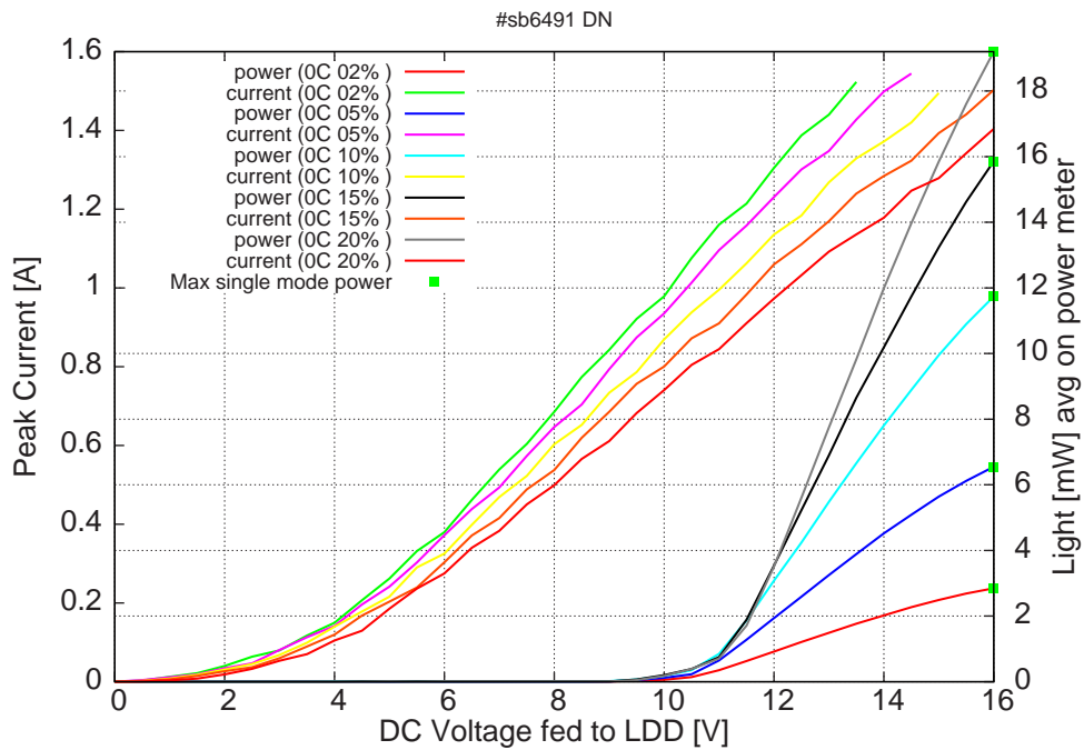
Figure 11: peak current and average power vs LDD voltage at 0C for various duty-cycles (100ns pulses on the laser) (the solid squares indicate the maximum singlemode emitted power)
