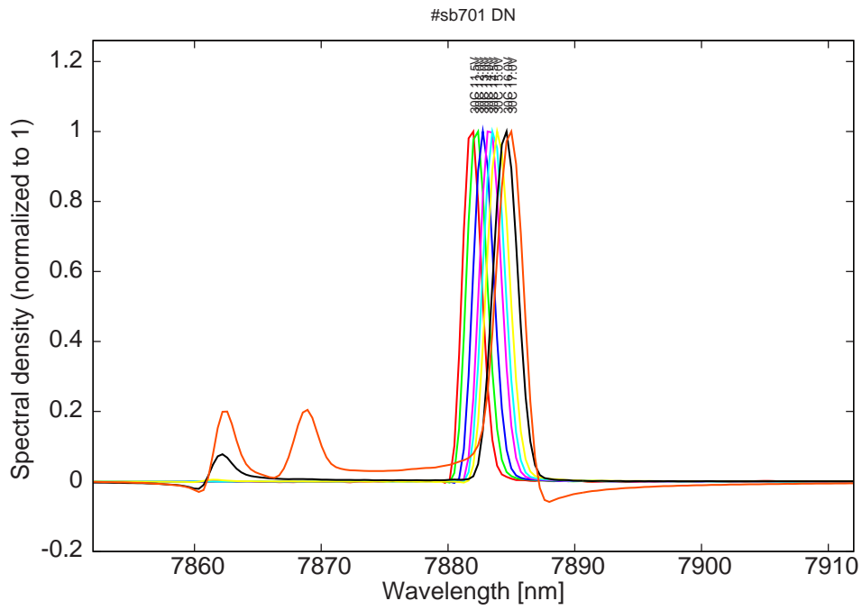
Figure 17: spectra at 30C for various LDD voltages
