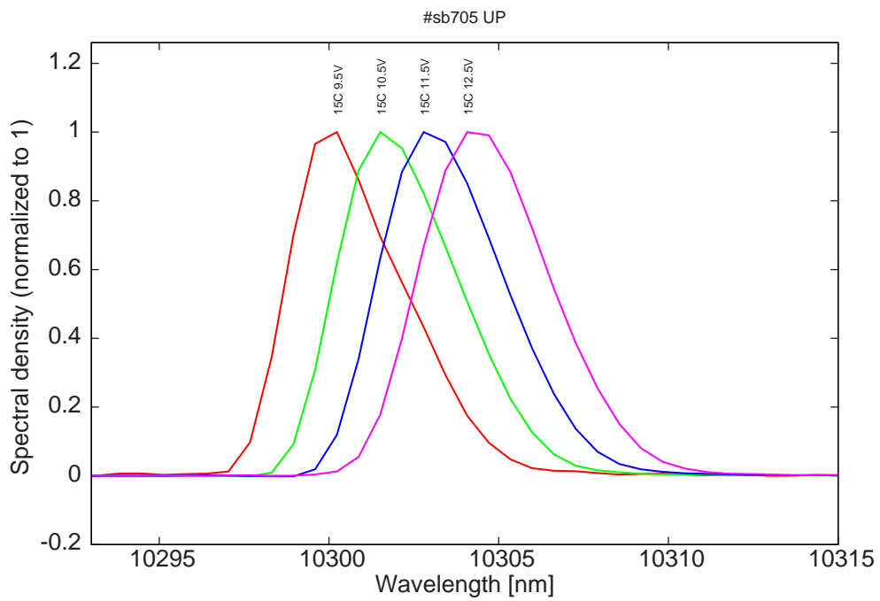
Figure 14: spectra at 15C for various LDD voltages
