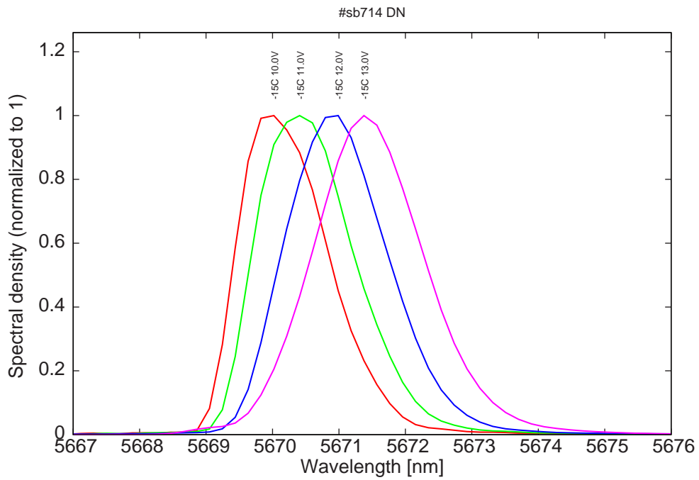
Figure 12: spectra at -15C for various LDD voltages (monomode range)
