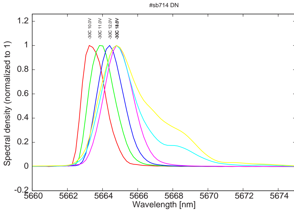
Figure 9: spectra at -30C for various LDD voltages (monomode up to 13V)
