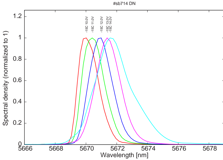
Figure 11: spectra at -15C for various LDD voltages (monomode up to 13V)
