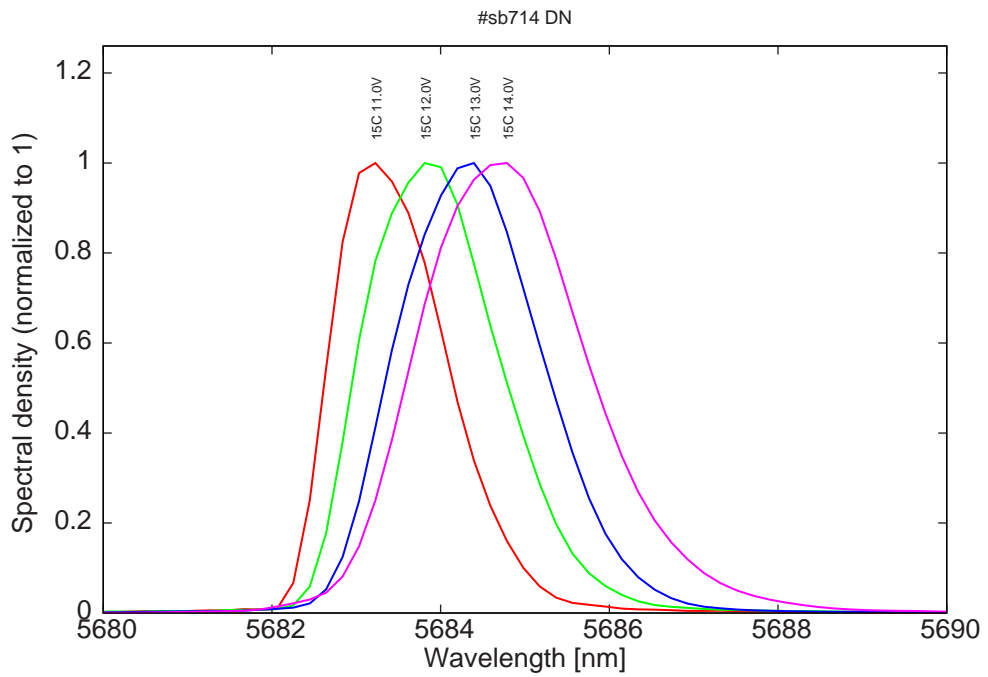
Figure 14: spectra at 15C for various LDD voltages (all monomode)
