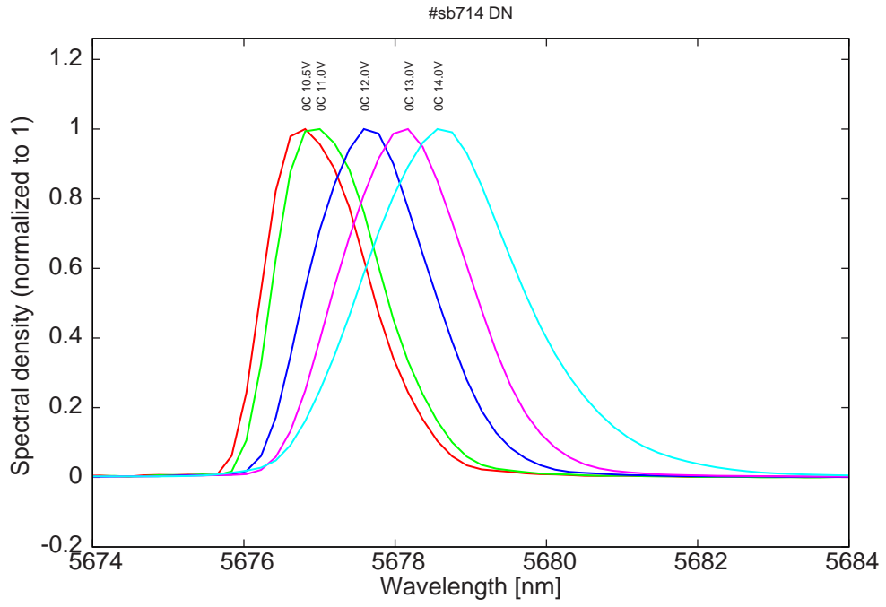
Figure 13: spectra at 0C for various LDD voltages (all monomode)
