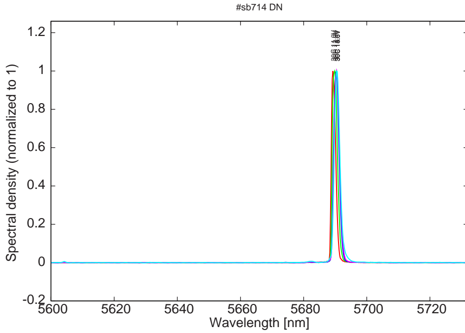
Figure 15: spectra at 30C for various LDD voltages (small mode around 5602nm)
