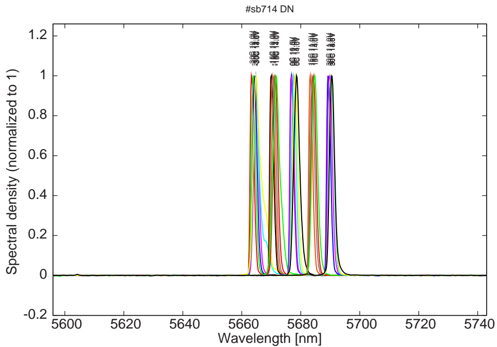
Figure 8: spectra at -30C, -15C, 0C, 15C and 30C at 2% dc for various LDD voltages (small mode around 5602nm)
