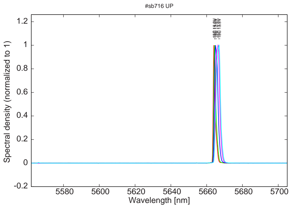
Figure 10: spectra at -15C for various LDD voltages (bimode a 13.5V, small mode around 5566nm)
