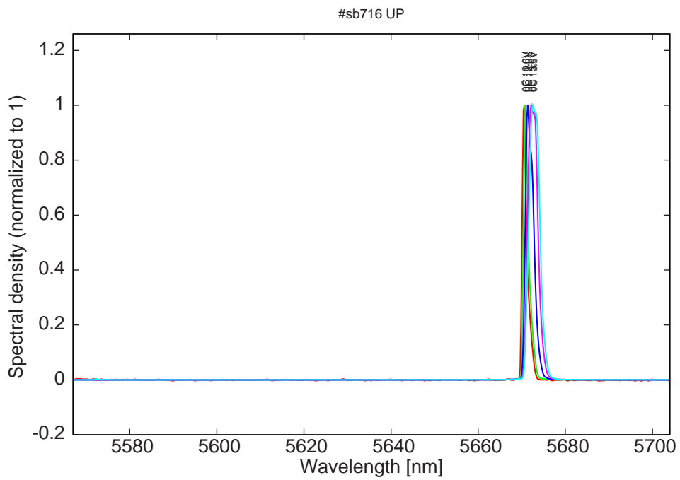
Figure 12: spectra at 0C for various LDD voltages (bimode at 13.5V, small mode around 5573nm)
