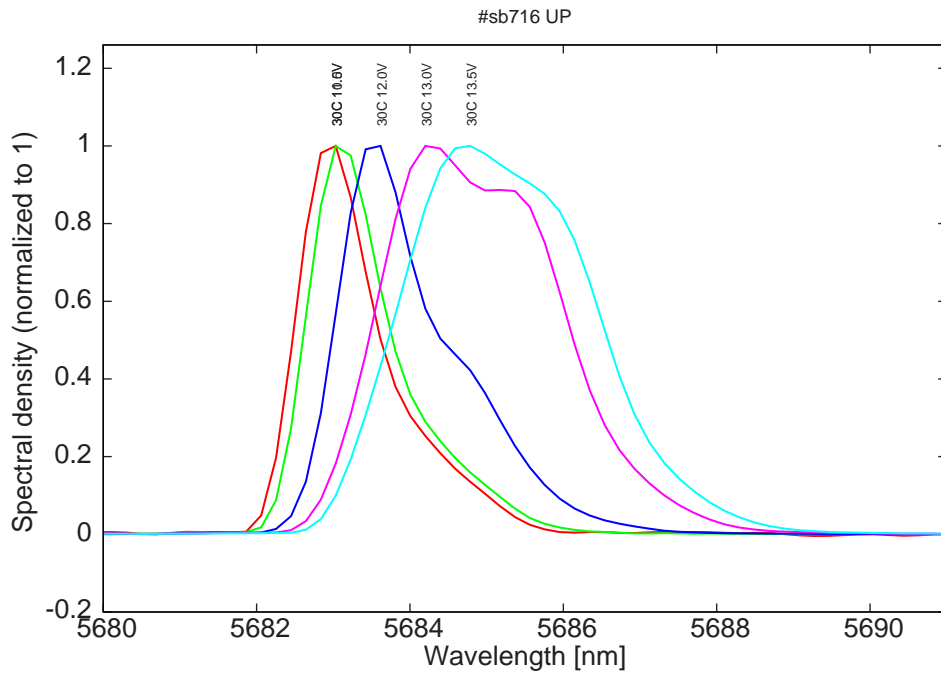
Figure 15: spectra at 30C for various LDD voltages (all monomode)
