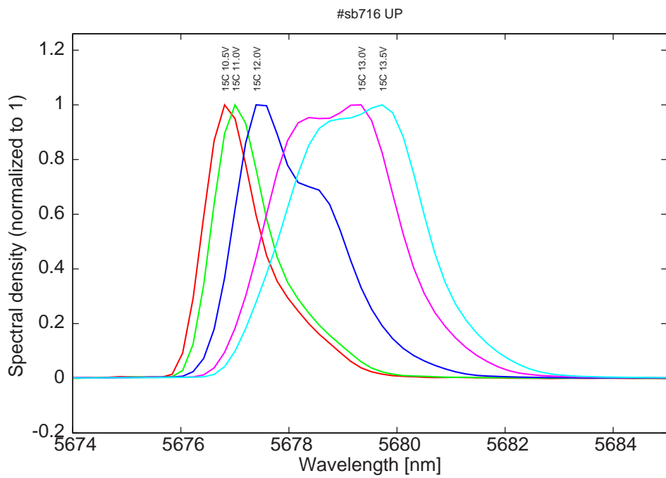
Figure 14: spectra at 15C for various LDD voltages (all monomode)
