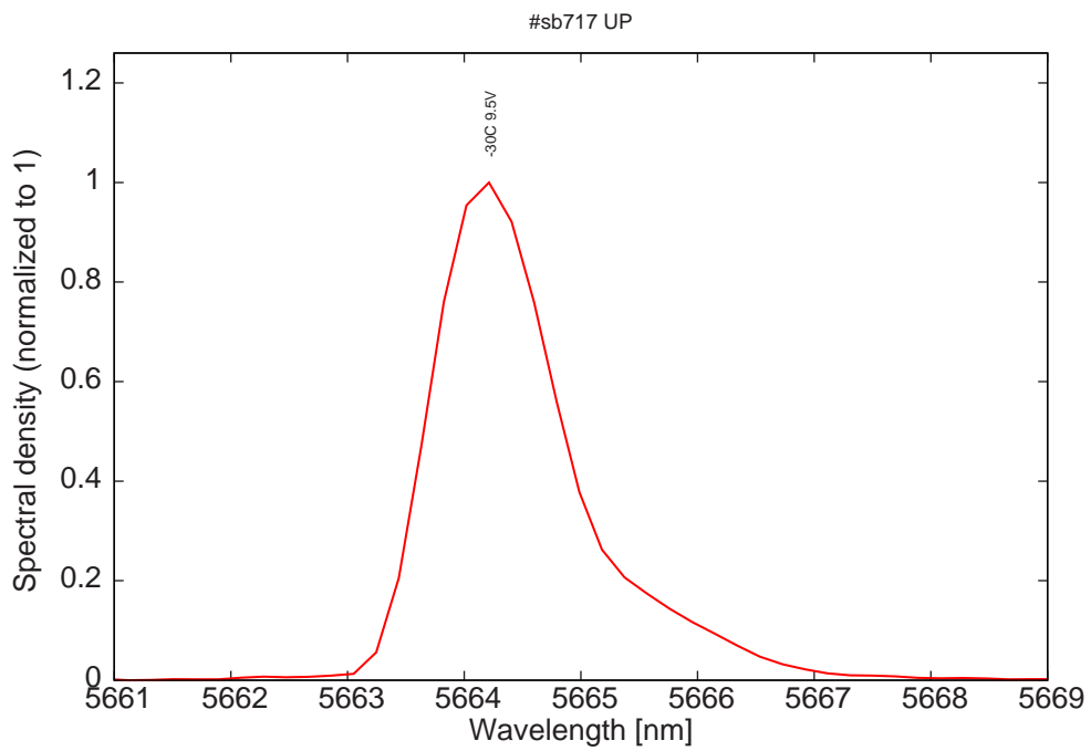
Figure 10: monomode spectrum at -30C and 9.5V on LDD
