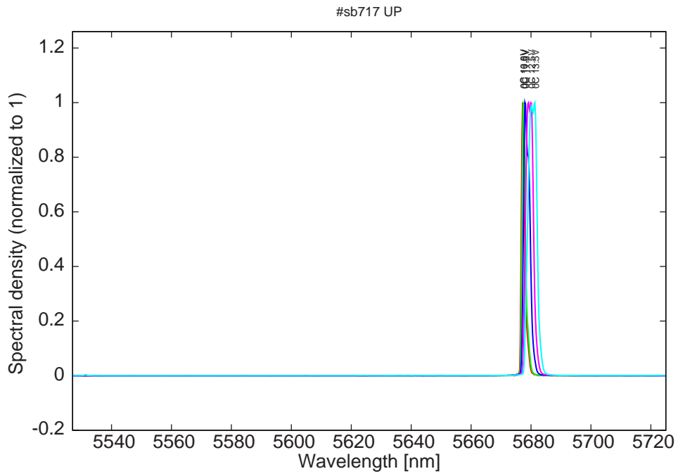
Figure 13: spectra at 0C for various LDD voltages (monomode up to 12.5V)
