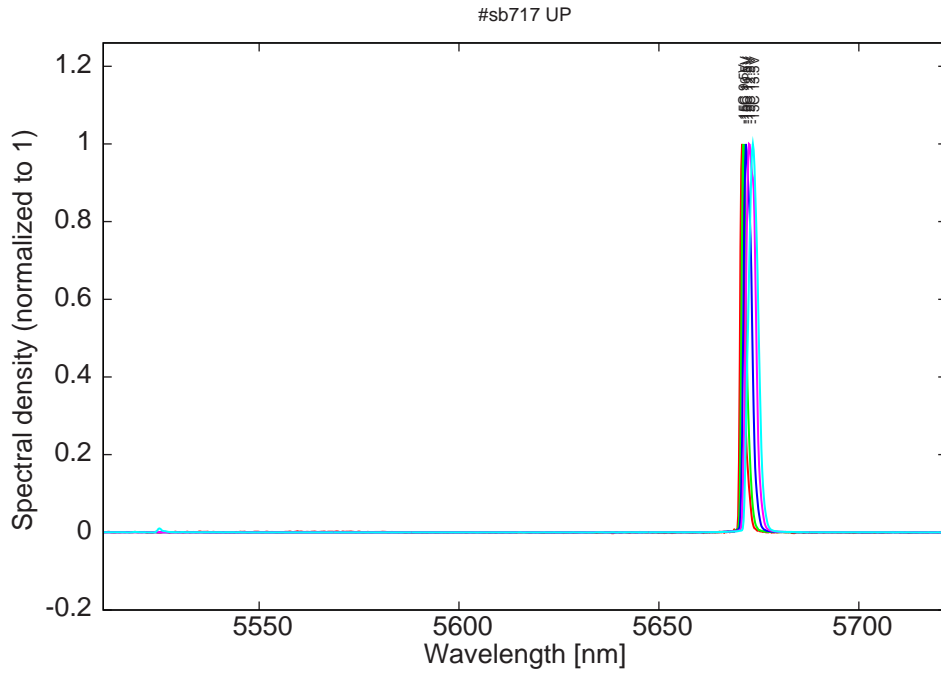
Figure 11: spectra at -15C for various LDD voltages (monomode up to 10.5V)
