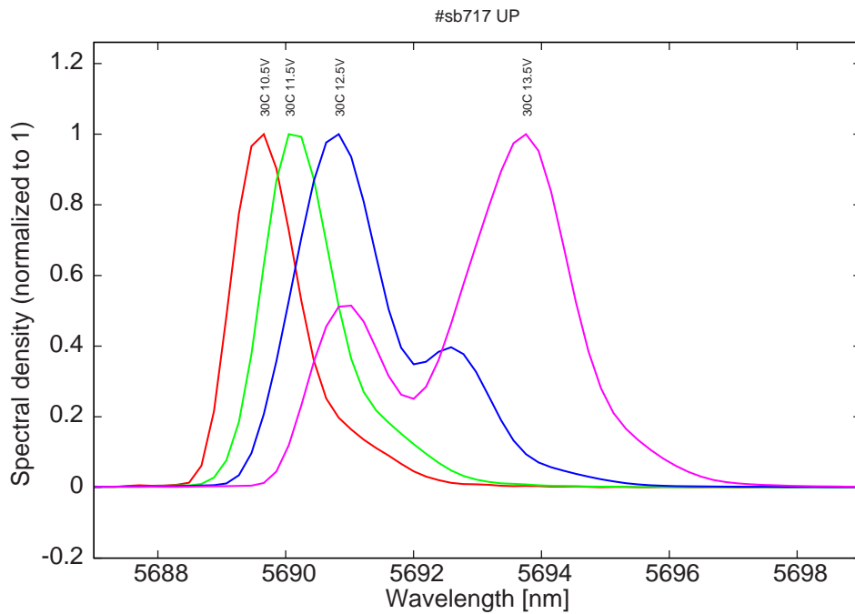
Figure 16: spectra at 30C for various LDD voltages (all monomode, holes due to absorption in the air at 5692nm)
