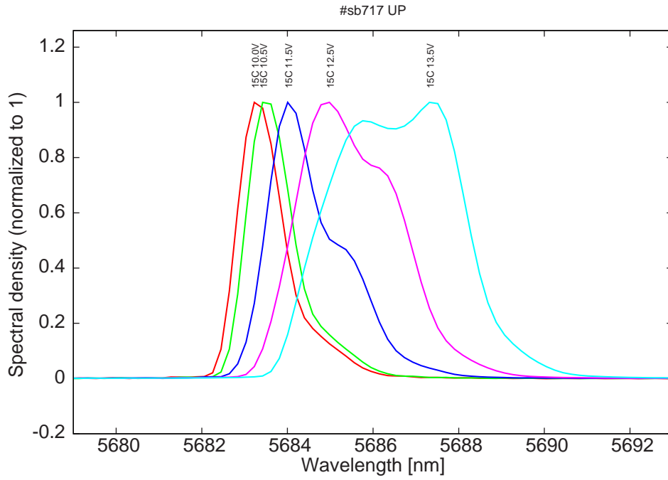
Figure 15: spectra at 15C for various LDD voltages (all monomode, holes due to absorption in the air)
