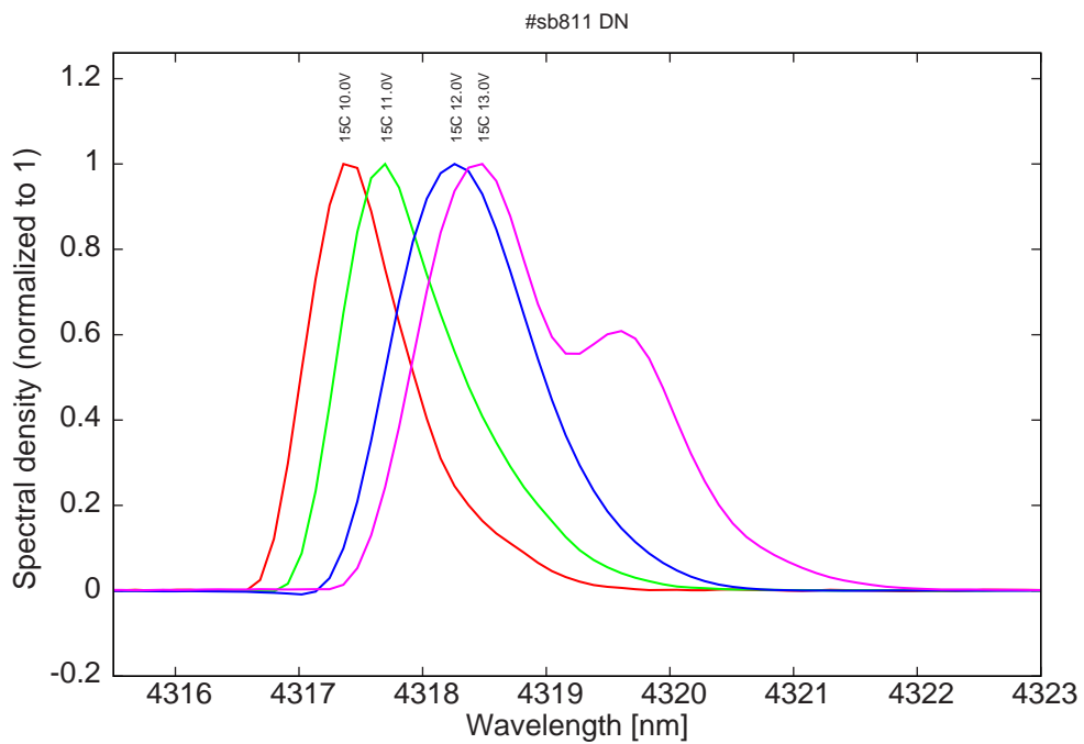
Figure 10: spectra at 15C for various LDD voltages (holes in the spectra due to absorption in the air around 4319.3nm )
