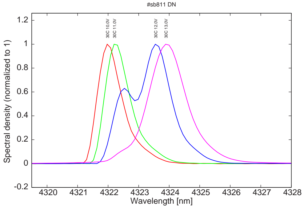
Figure 11: spectra at 30C for various LDD voltages (holes in the spectra due to absorption in the air around 4323nm)
