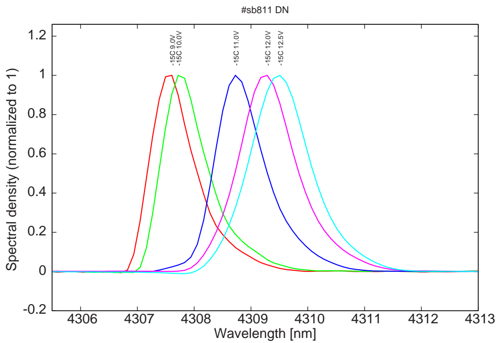
Figure 8: spectra at -15C for various LDD voltages (absorption in the air around 4308.3nm)
