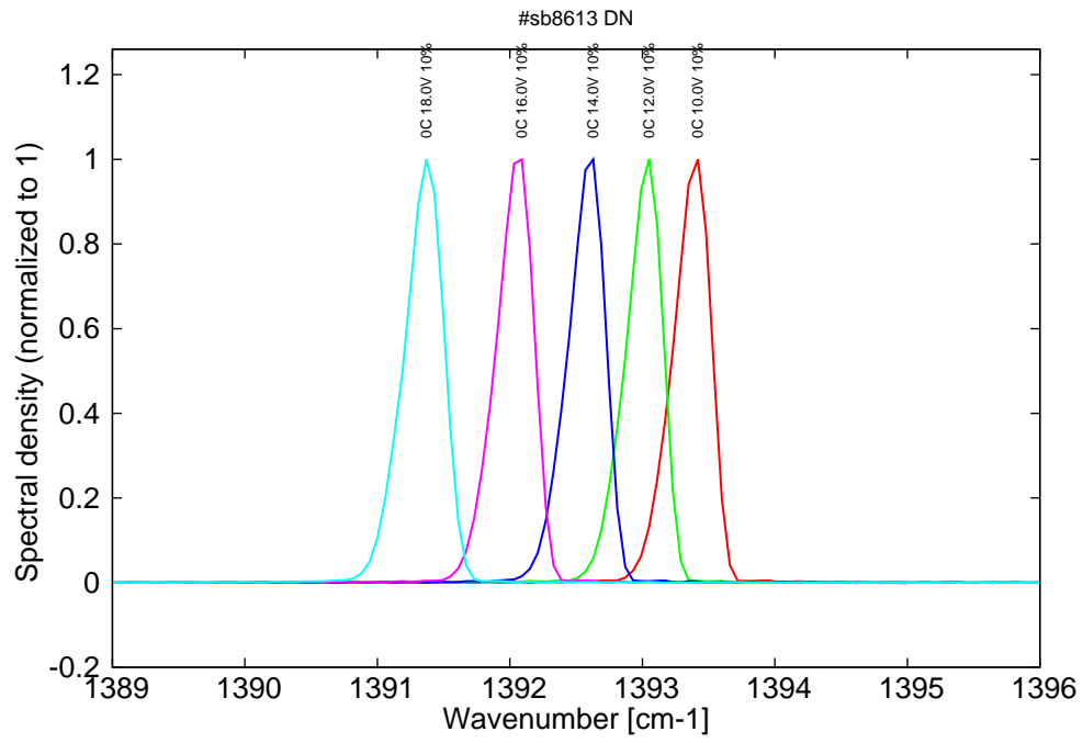
Figure 8: spectra at 0C at 10%dc for various LDD voltages
