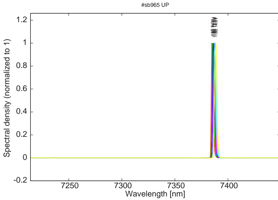
Figure 11: spectra at -15C for various LDD voltages (small mode around 7234nm at 13.0V and 14.0V on LDD)
