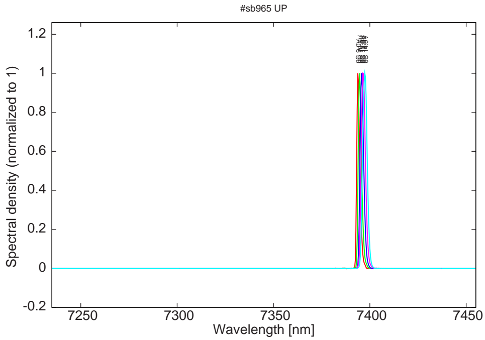
Figure 13: spectra at 0C for various LDD voltages (small mode around 7243nm at 14.0V on LDD)
