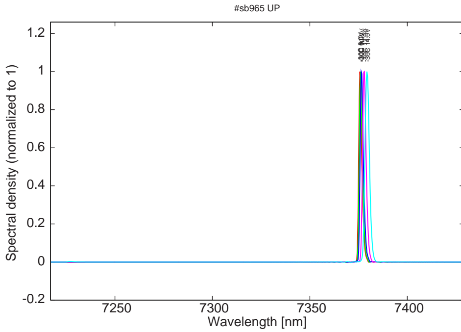
Figure 9: spectra at -30C for various LDD voltages (small mode around 7225nm at 14.0V on LDD)
