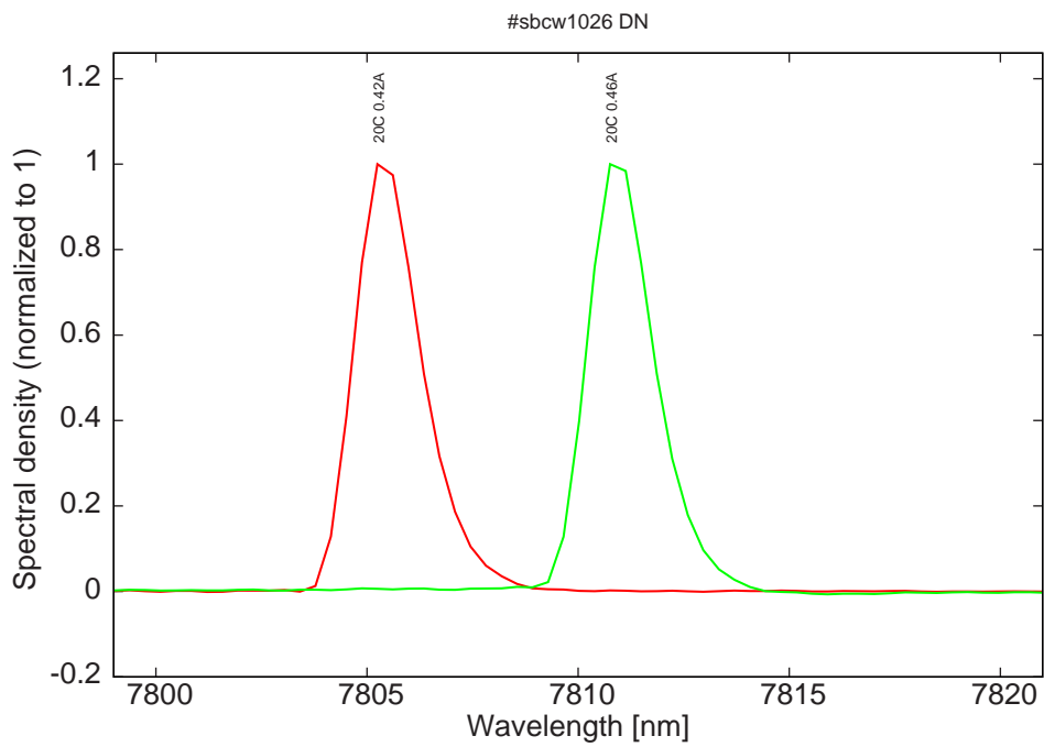
Figure 10: spectra at 20C for various DC currents
