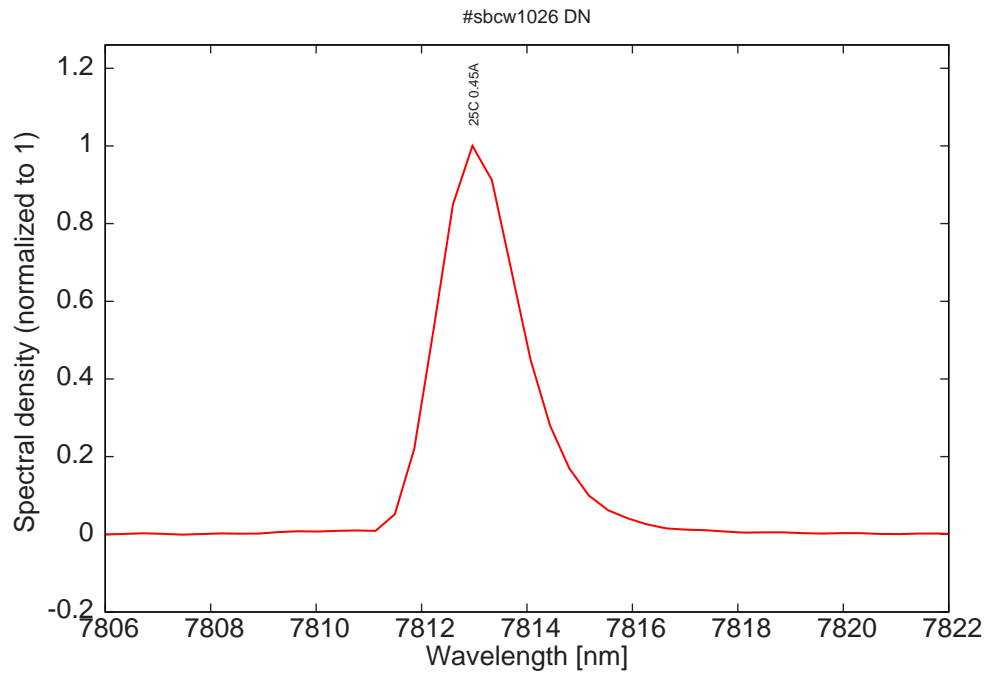
Figure 11: monomode spectrum at 25C and 0.45A
