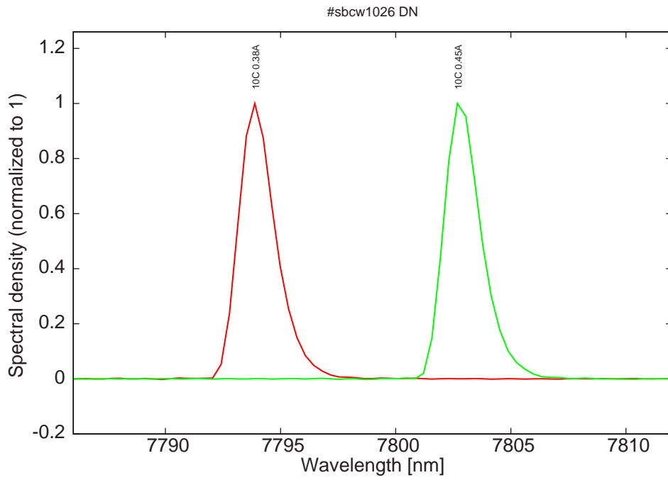
Figure 9: spectra at 10C for various DC currents
