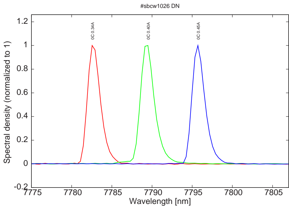
Figure 8: spectra at 0C for various DC currents
