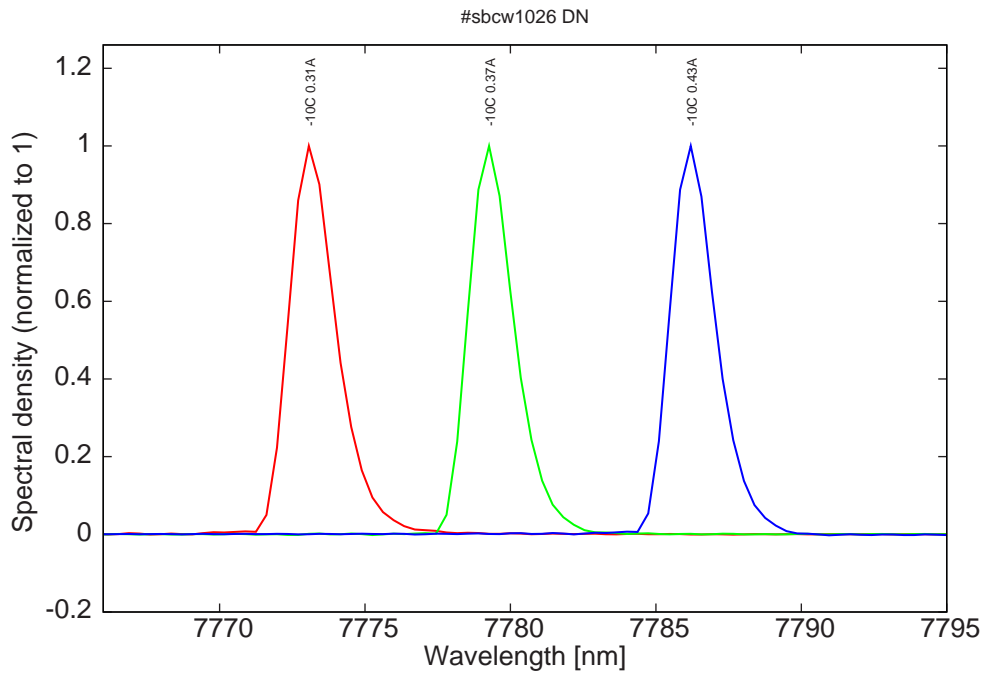
Figure 7: spectra at -10C for various DC currents
