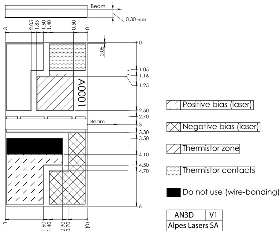
Figure 1: Support mounting for #sbcw10554 DN (please note that AlN submount numbering is P0226)
