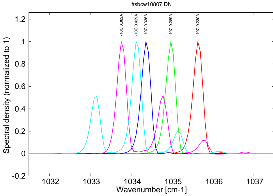
Figure 8: spectra at -10C for various DC current (monomode up to 0.335A, then becomes multimode)
