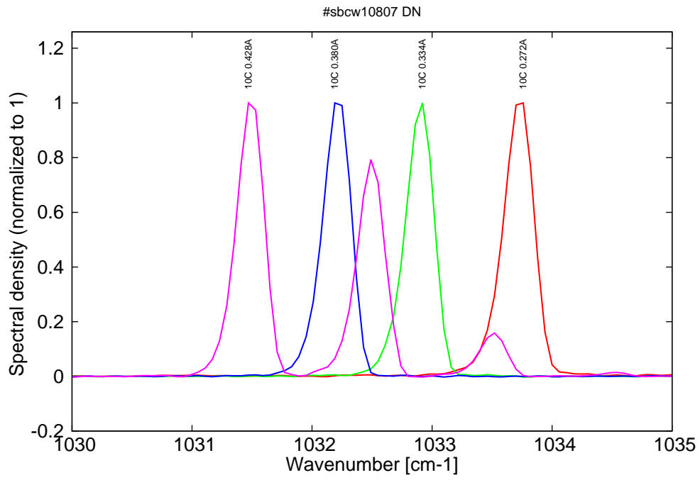
Figure 10: spectra at 10C for various DC current (monomode up to 0.38A, then becomes multimode)
