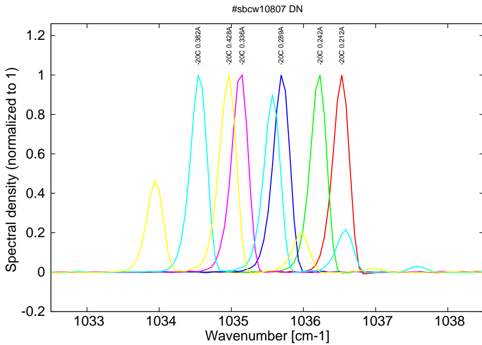
Figure 7: spectra at -20C for various DC current (monomode up to 0.335A, then becomes multimode)
