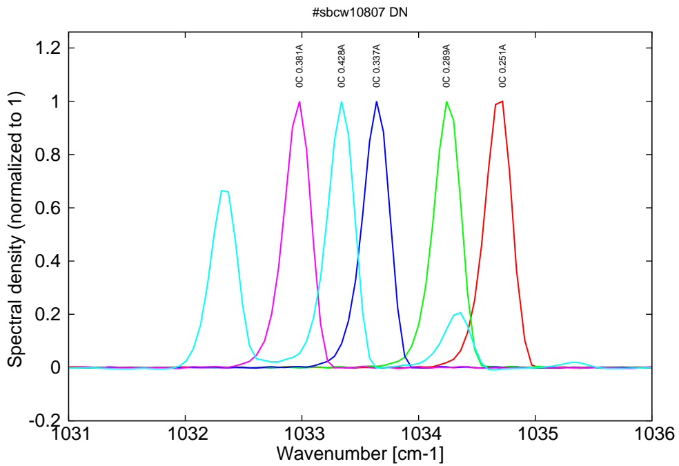
Figure 9: spectra at 0C for various DC current (monomode up to 0.38A, then becomes multimode)
