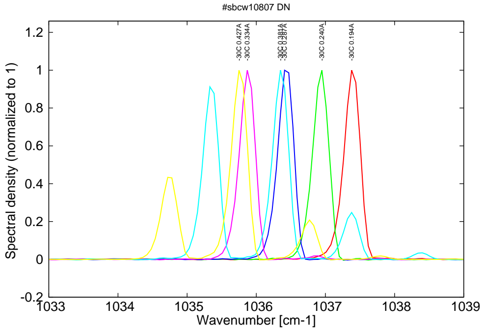
Figure 6: spectra at -30C for various DC current (monomode up to 0.29A, then becomes multimode)
