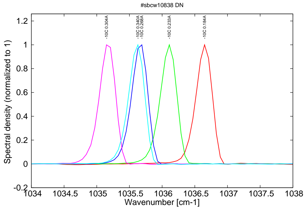
Figure 7: spectra at -10C for various DC currents (monomode on mode 1 up to 0.30A, then becomes monomode on mode 2)
