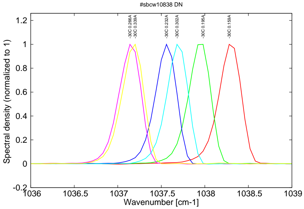
Figure 5: spectra at -30C for various DC currents (monomode on mode 1 up to 0.265A, then becomes monomode on mode 2)
