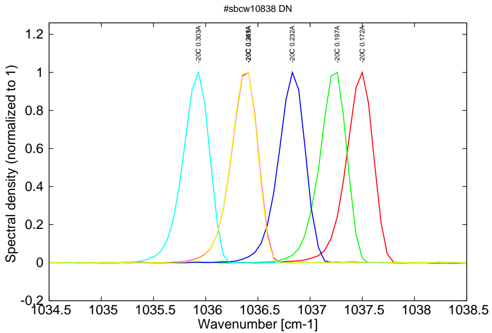
Figure 6: spectra at -20C for various DC currents (monomode on mode 1 up to 0.30A, then becomes monomode on mode 2)
