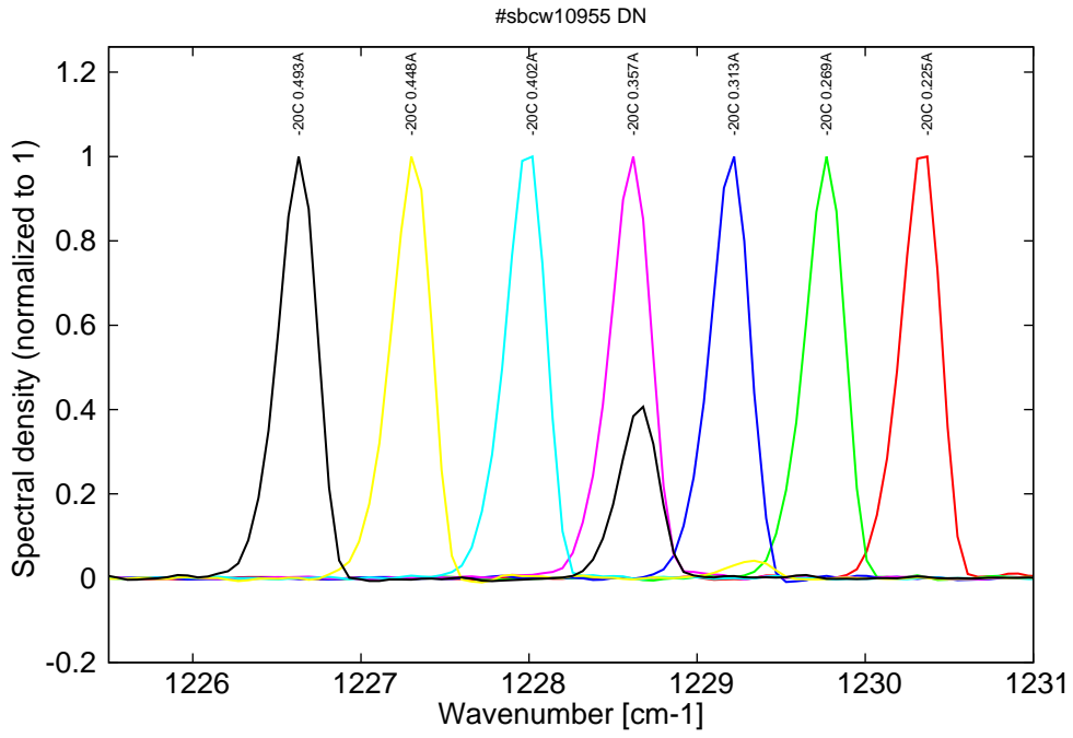
Figure 6: spectra at -20C for various DC currents (monomode up to 0.4A, then becomes bimode)
