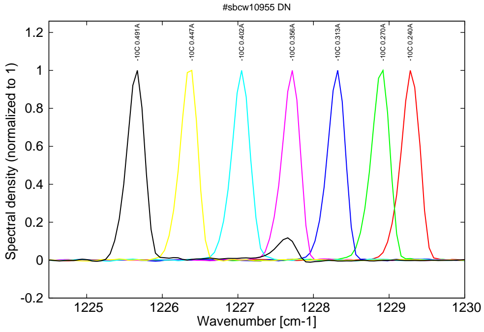
Figure 8: spectra at -10C for various DC currents (monomode up to 0.445A, then becomes bimode)
