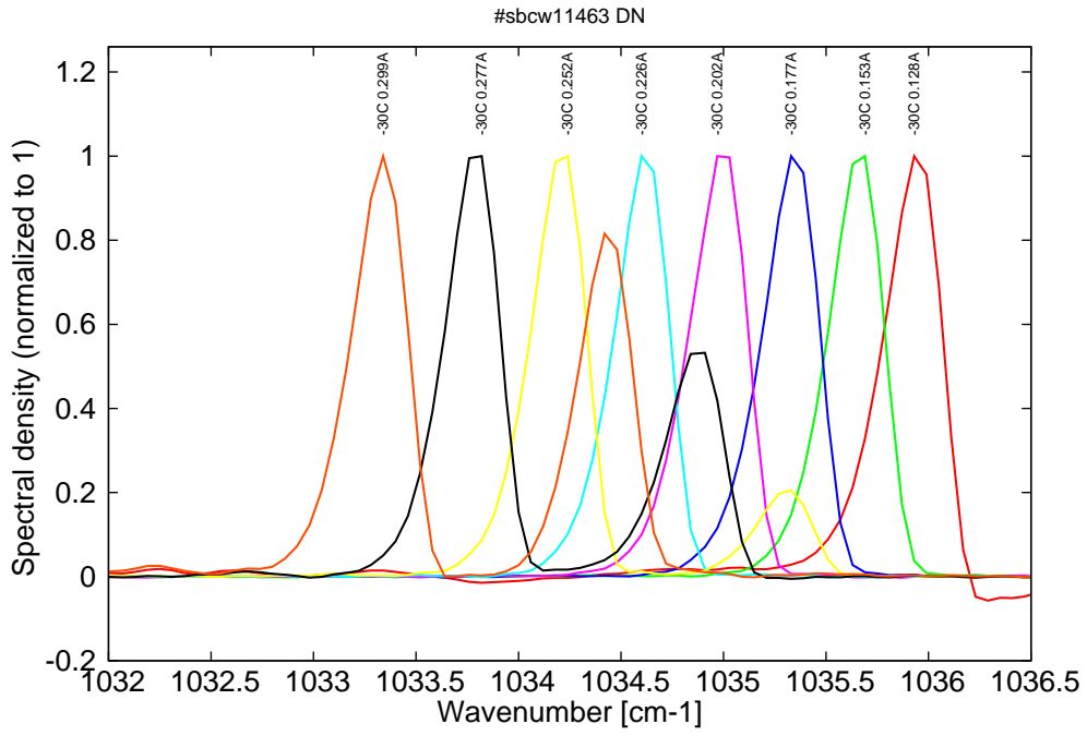
Figure 6: spectra at -30C for various DC currents (monomode up to 0.225A, then becomes bimode)
