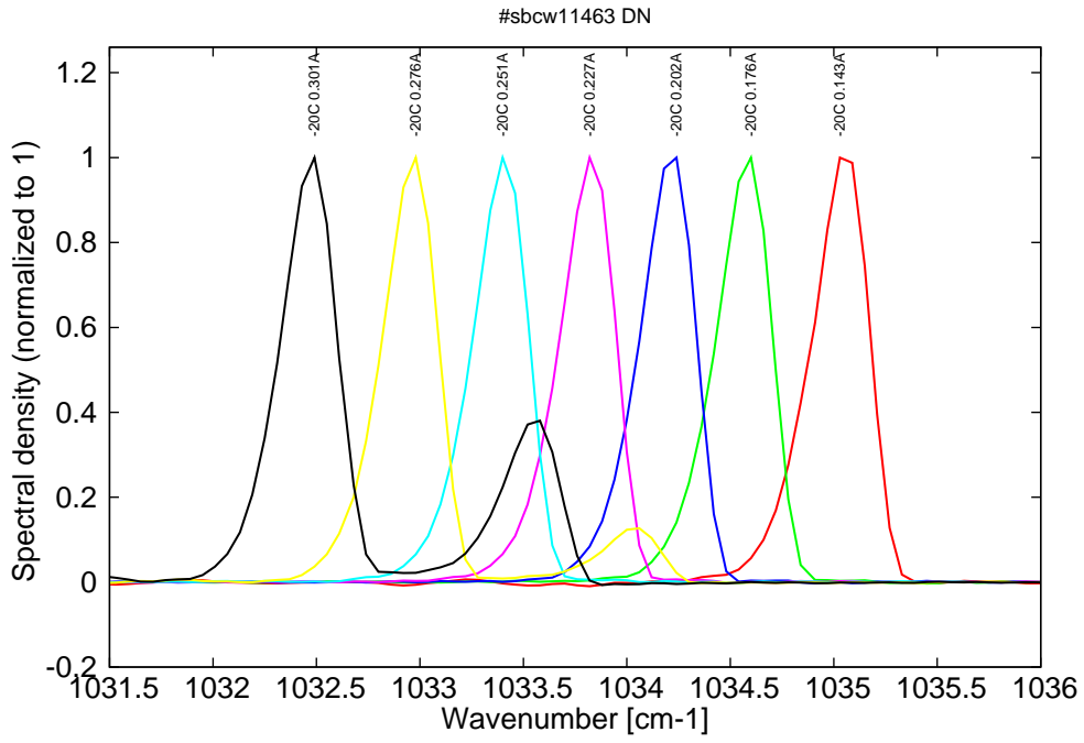
Figure 8: spectra at -20C for various DC currents (monomode up to 0.25A, then becomes bimode)
