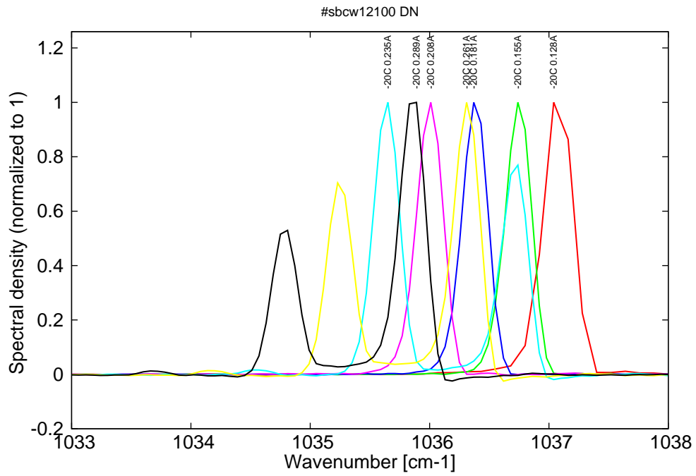
Figure 6: spectra at -20C for various DC currents (monomode up to 0.18A, then becomes multimode)
