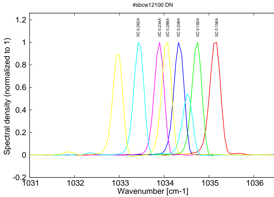
Figure 10: spectra at 0C for various DC currents (monomode up to 0.23A, then becomes multimode)
