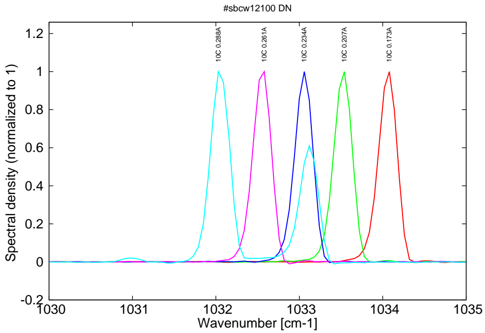
Figure 12: spectra at 10C for various DC currents (monomode up to 0.26A, then becomes multimode)
