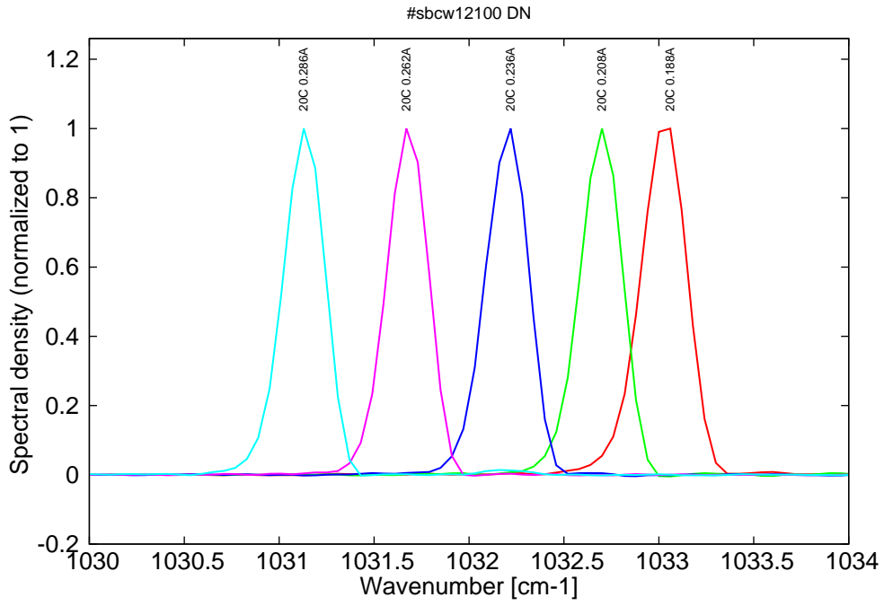
Figure 14: spectra at 20C for various DC currents (monomode up to 0.26A, then becomes bimode)
