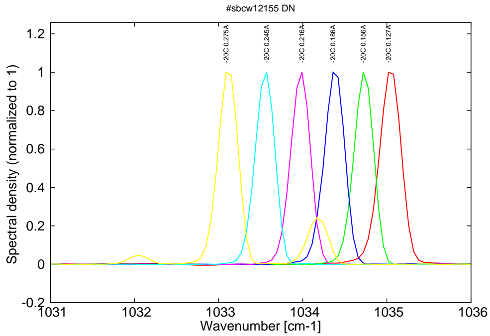
Figure 6: spectra at -20C for various DC currents (monomode up to 0.245A, then multi-mode)
