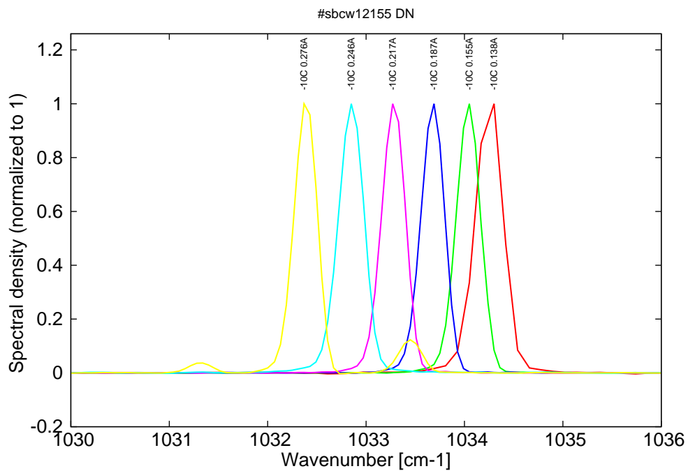
Figure 7: spectra at -10C for various DC currents (monomode up to 0.245A, then multi-mode)
