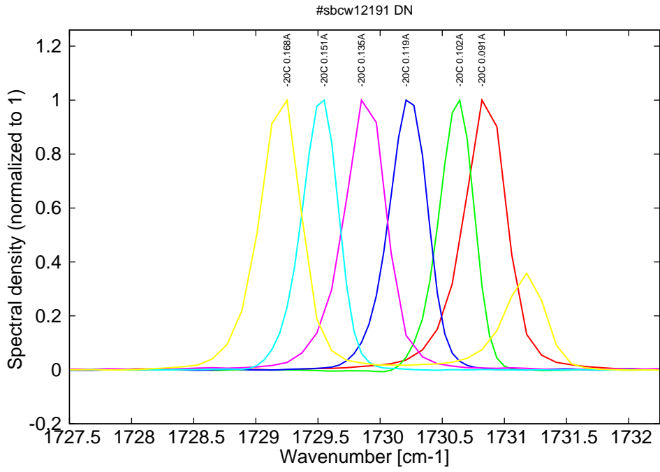
Figure 8: spectra at -20C for various DC currents (monomode up to 0.15A then becomes bimode)
