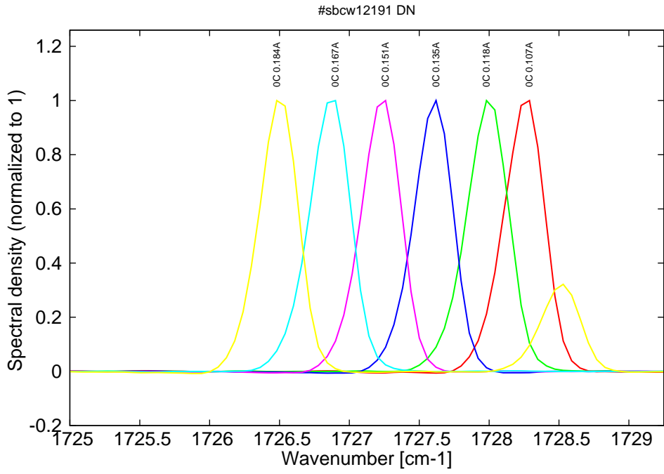
Figure 12: spectra at 0C for various DC currents (monomode up to 0.165A then becomes bimode)
