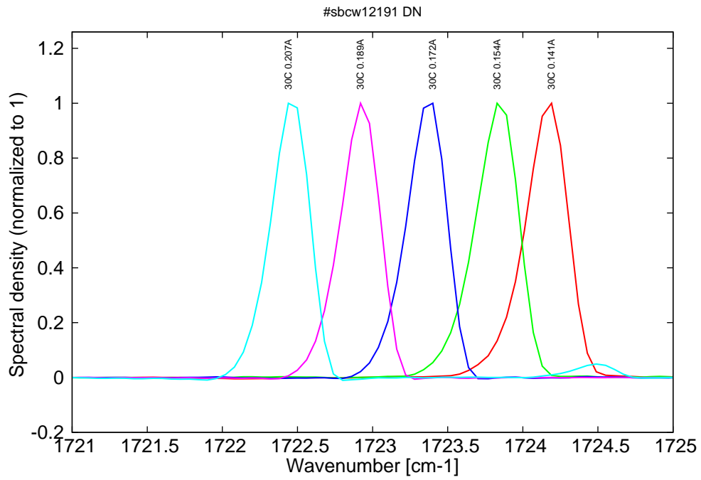
Figure 20: spectra at 30C for various DC currents (monomode up to 0.185A then becomes bimode)
