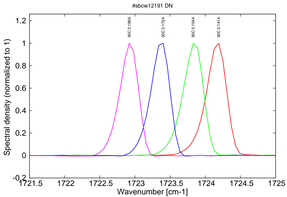
Figure 21: spectra at 30C for various DC currents (monomode range)
