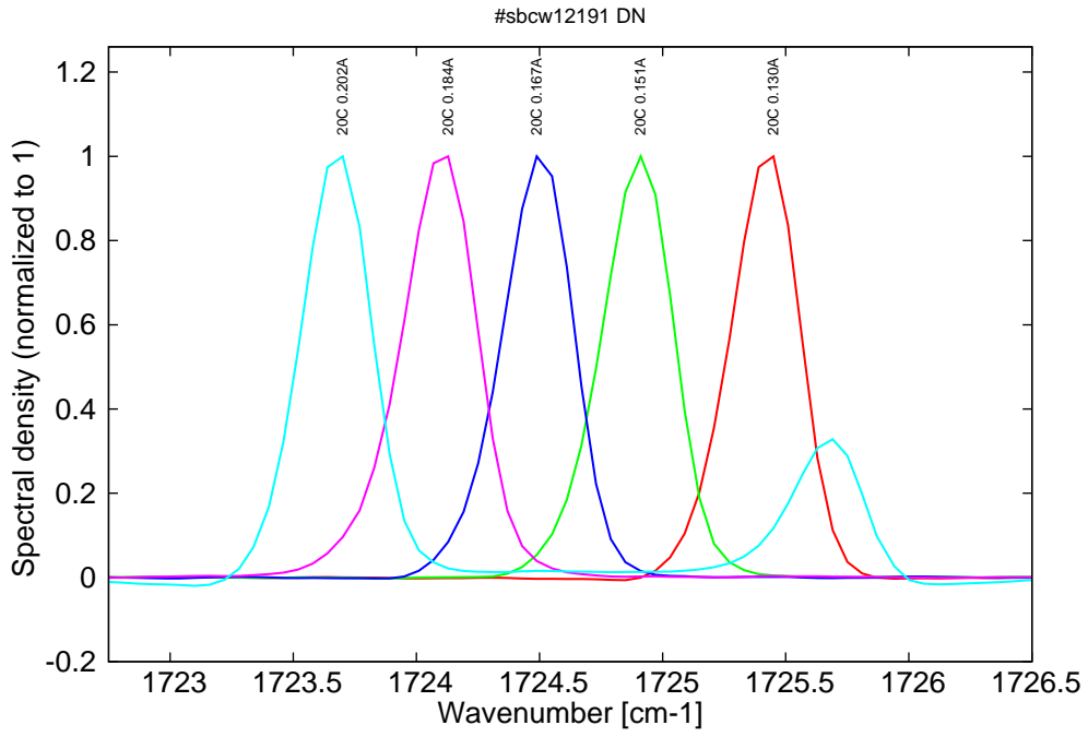
Figure 16: spectra at 20C for various DC currents (monomode up to 0.185A then becomes bimode)
