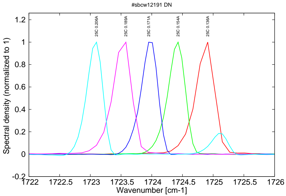
Figure 18: spectra at 25C for various DC currents (monomode up to 0.185A then becomes bimode)
