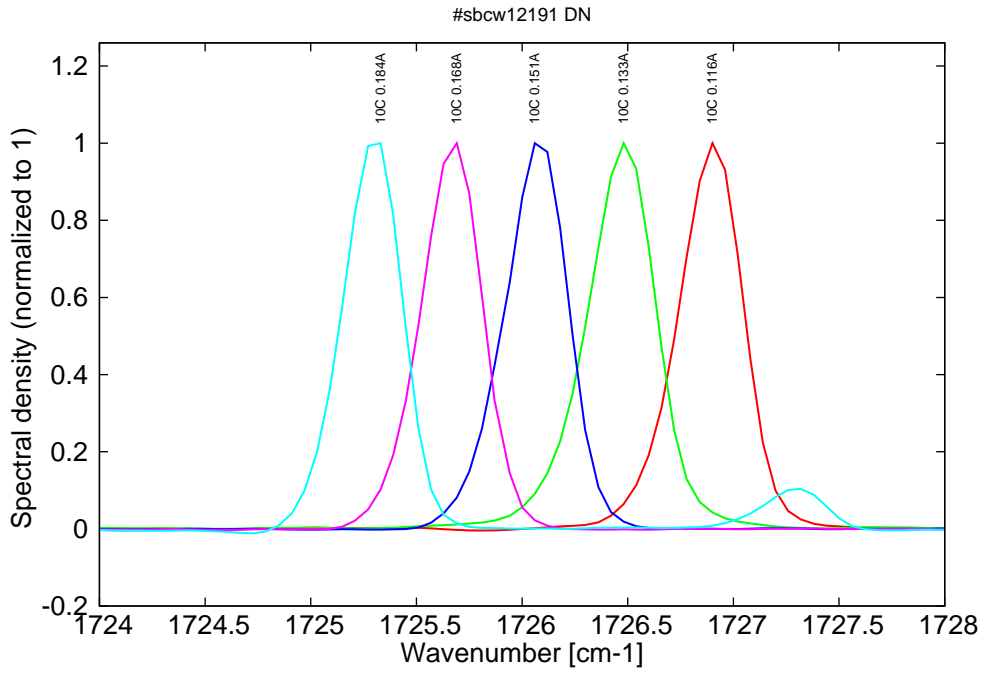
Figure 14: spectra at 10C for various DC currents (monomode up to 0.165A then becomes bimode)
