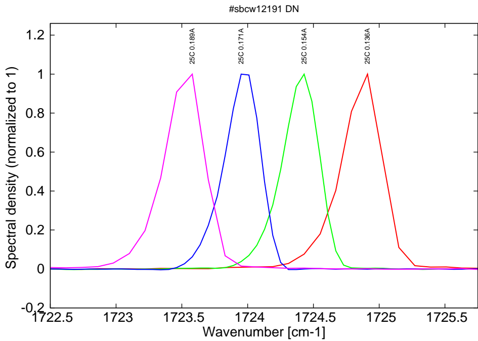
Figure 19: spectra at 25C for various DC currents (monomode range)
