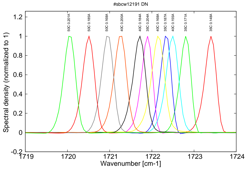
Figure 22: spectra between 35C and 50C for various DC currents (all monomode)
