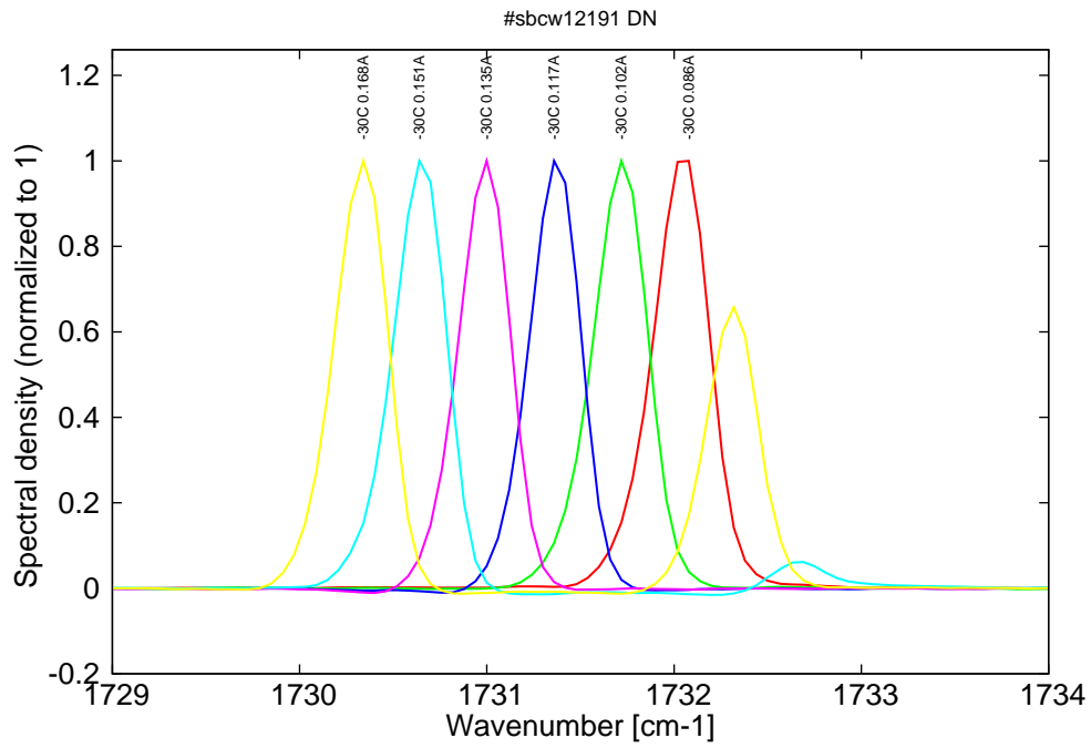
Figure 6: spectra at -30C for various DC currents (monomode up to 0.135A then becomes bimode)
