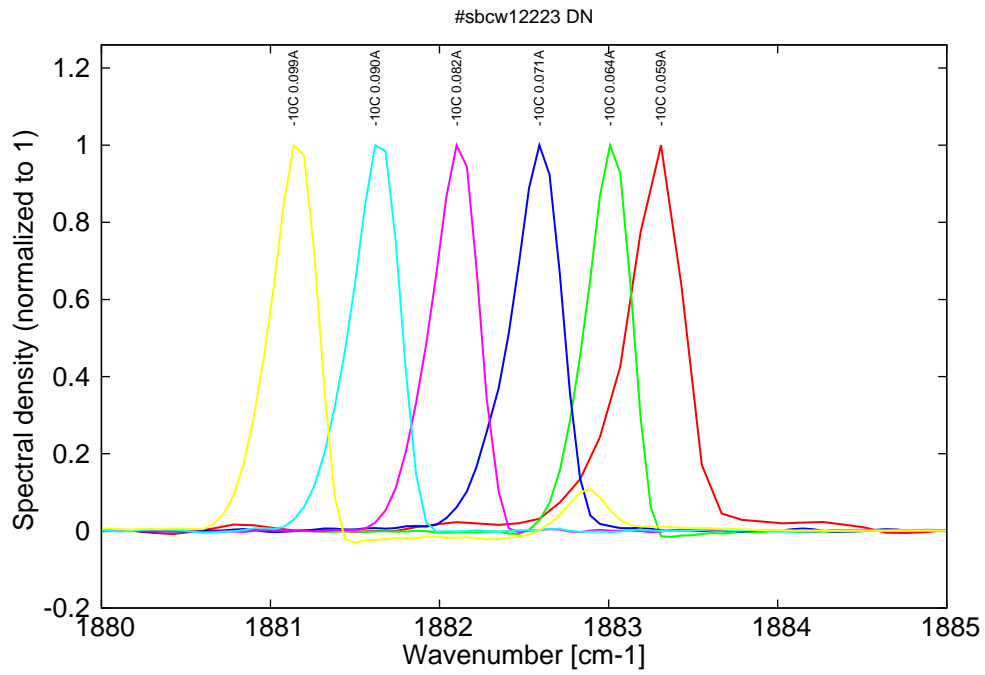
Figure 8: spectra at -10C for various DC currents (monomode up to 0.09A, then becomes bimode)
