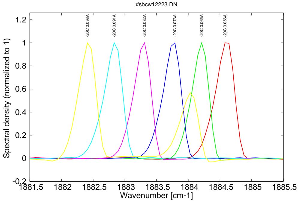
Figure 6: spectra at -20C for various DC currents (monomode up to 0.09A, then becomes bimode)
