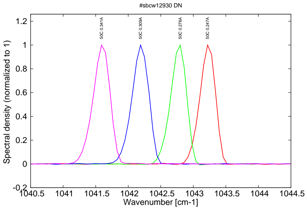
Figure 13: spectra at 50C for various DC currents (monomode up to 0.34A)
