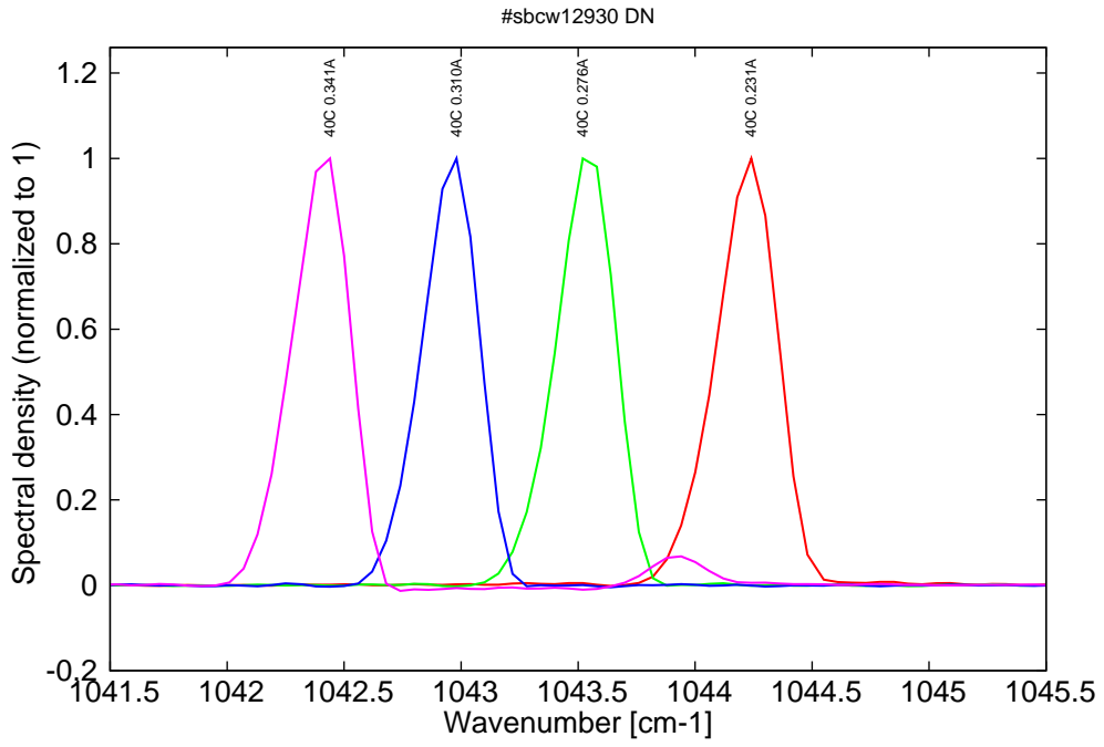
Figure 12: spectra at 40C for various DC currents (monomode up to 0.31A, then bimode)
