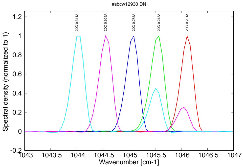
Figure 10: spectra at 20C for various DC currents (monomode up to 0.275A, then bimode)
