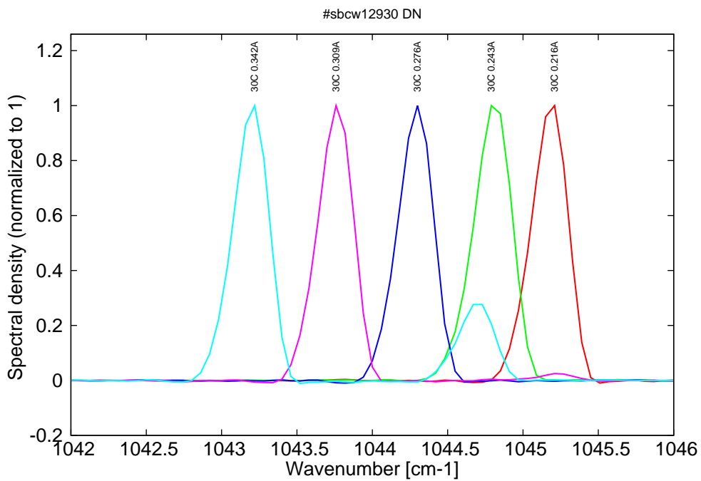
Figure 11: spectra at 30C for various DC currents (monomode up to 0.275A, then bimode)
