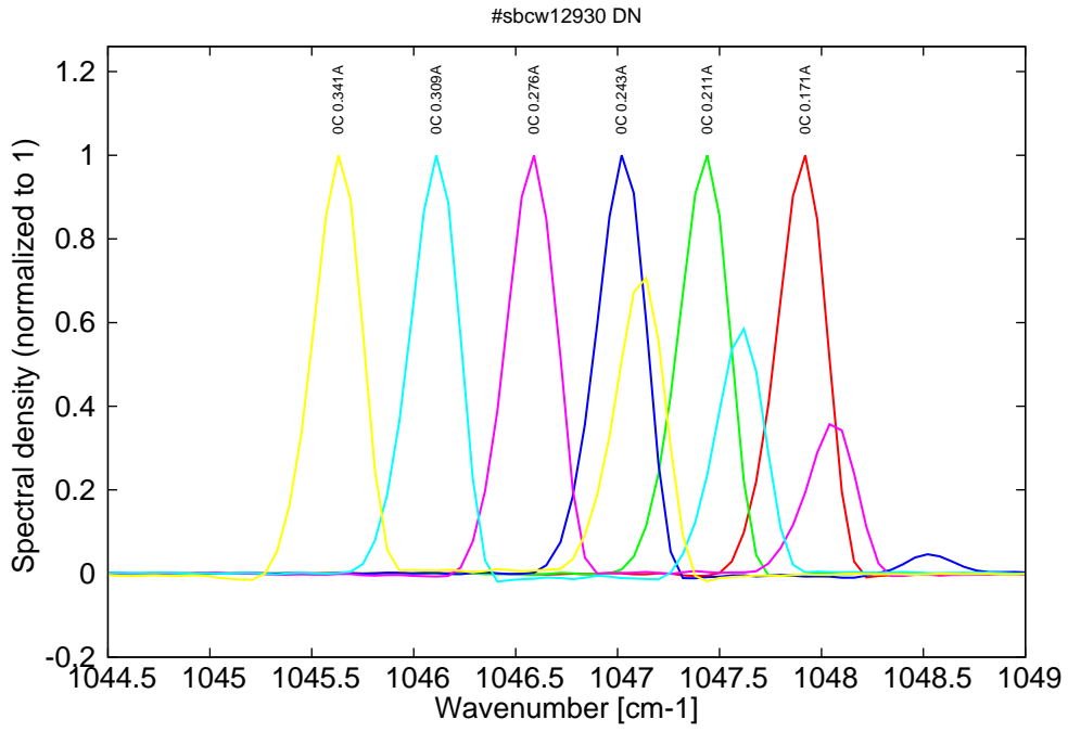
Figure 8: spectra at 0C for various DC currents (monomode up to 0.21A, then bimode)
