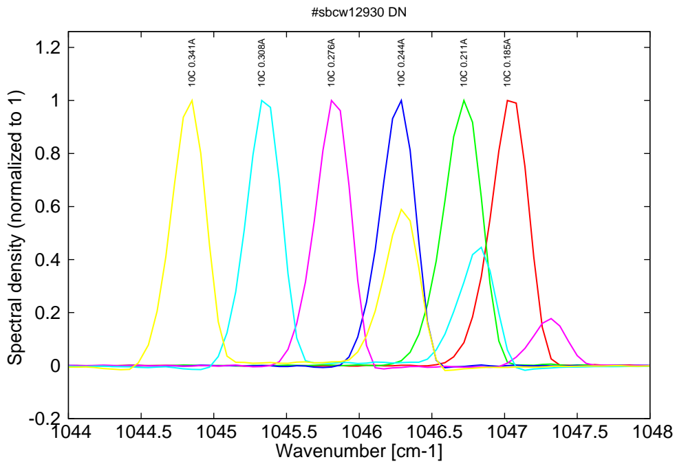
Figure 9: spectra at 10C for various DC currents (monomode up to 0.245A, then bimode)
