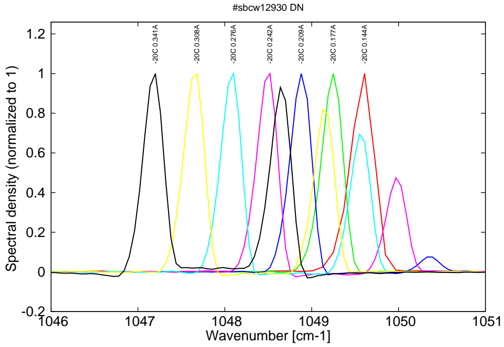
Figure 6: spectra at -20C for various DC currents (monomode up to 0.175A, then bimode)
