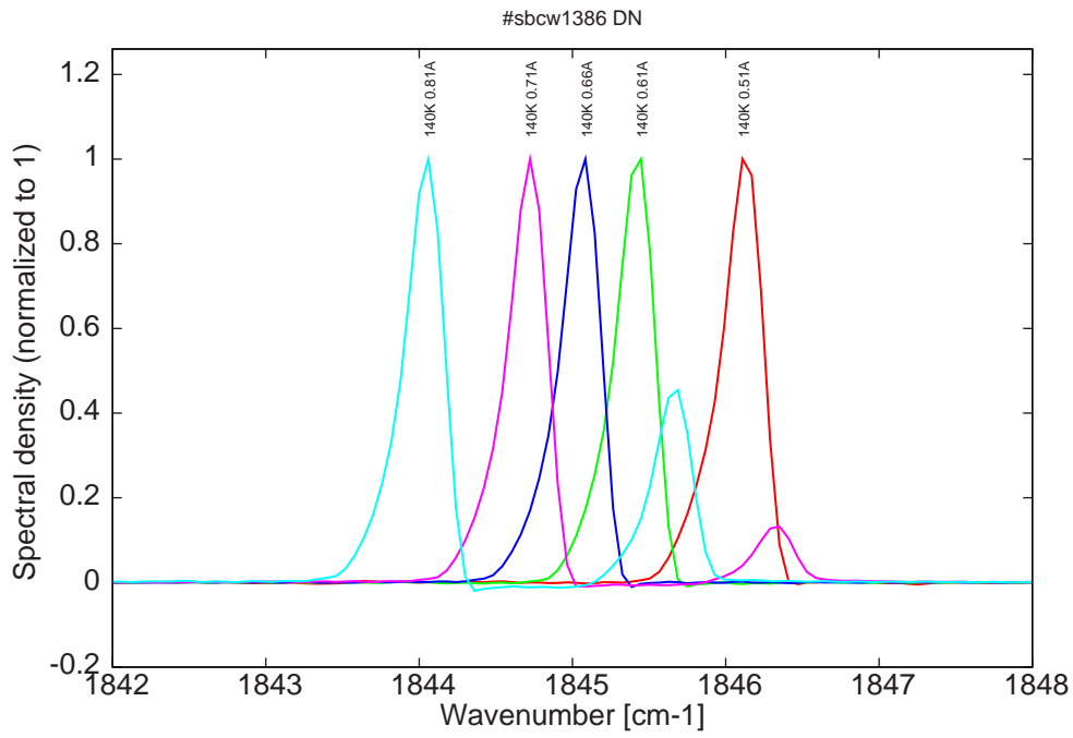
Figure 6: spectra at 140K for various DC currents (monomode up to 0.66A)
