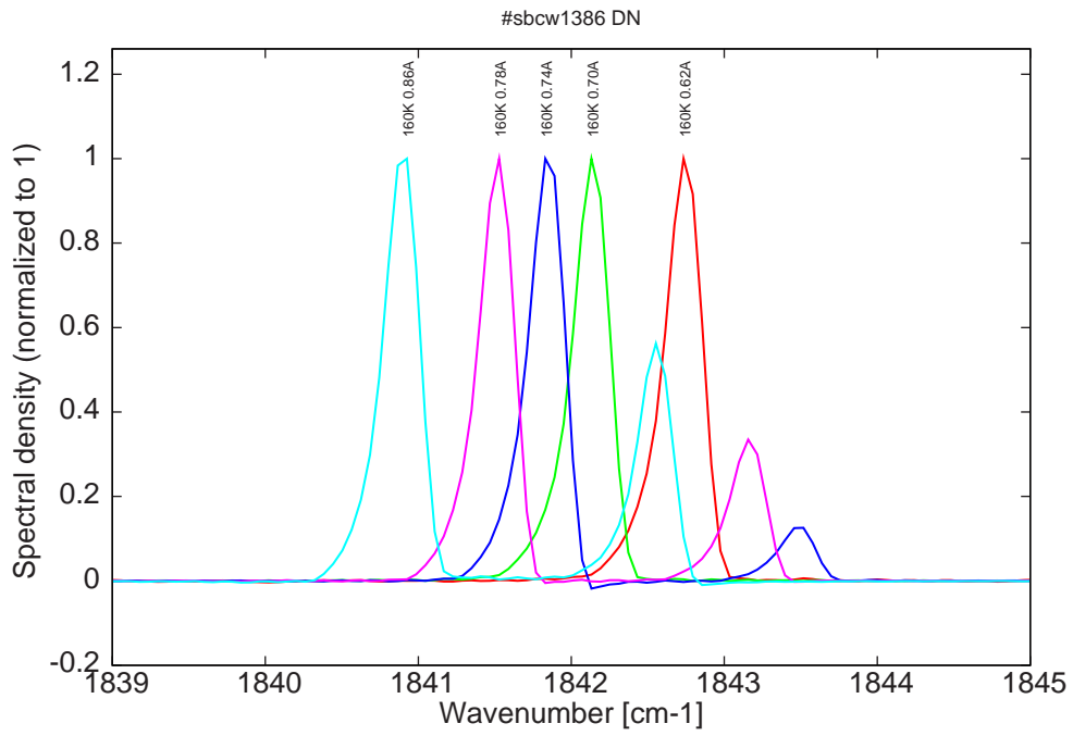
Figure 8: spectra at 160K for various DC currents (monomode up to 0.70A)
