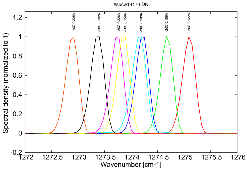
Figure 7: spectra at -20C and -10C for various DC currents (monomode range)
