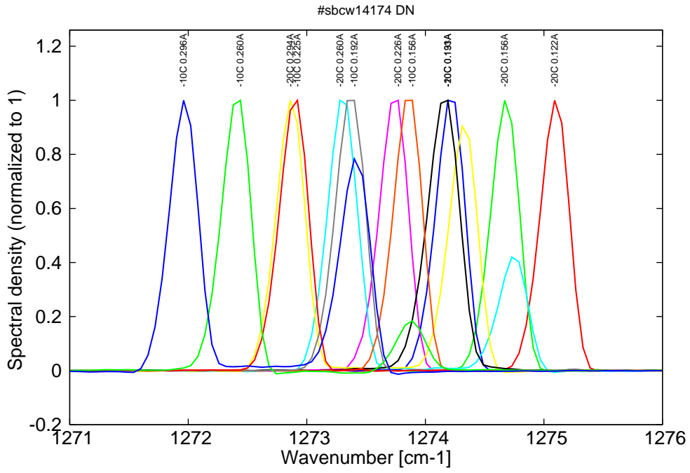
Figure 6: spectra at -20C and -10C for various DC currents (monomode up to 0.225A, then becomes bimode)
