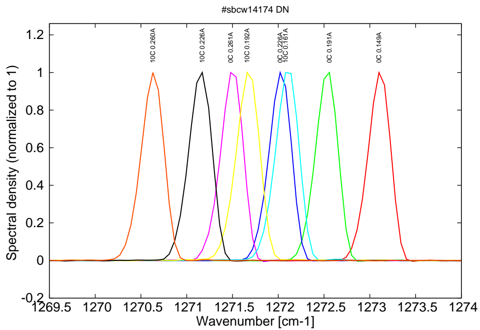
Figure 9: spectra at 0C and 10C for various DC currents (monomode range)
