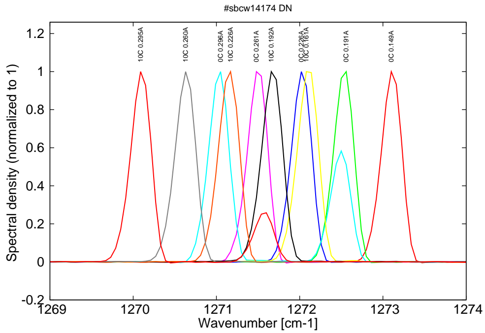
Figure 8: spectra at 0C and 10C for various DC currents (monomode up to 0.26A, then becomes bimode)
