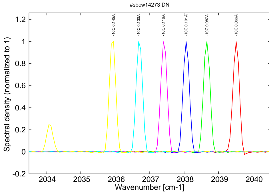
Figure 8: spectra at -10C for various DC currents (monomode up to 0.13A, then becomes bimode)
