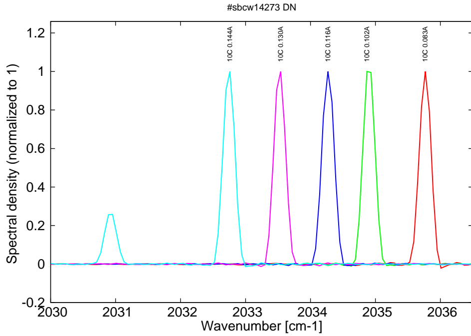
Figure 12: spectra at 10C for various DC currents (monomode up to 0.13A, then becomes bimode)
