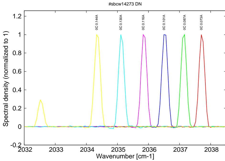
Figure 10: spectra at 0C for various DC currents (monomode up to 0.13A, then becomes bimode)
