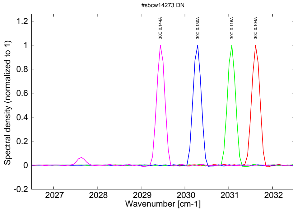
Figure 16: spectra at 30C for various DC currents (monomode up to 0.13A, then becomes bimode)
