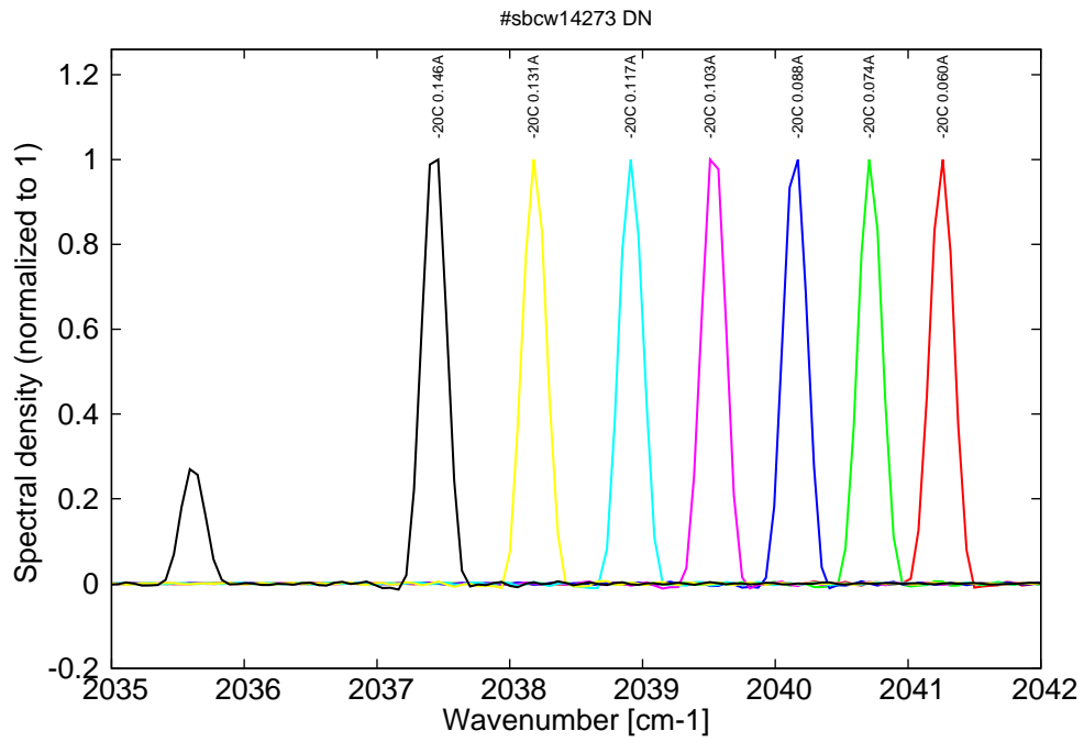
Figure 6: spectra at -20C for various DC currents (monomode up to 0.13A, then becomes bimode)
