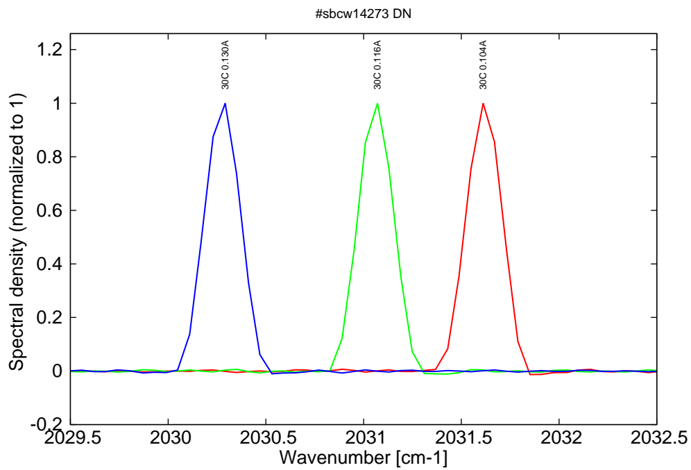
Figure 17: spectra at 30C for various DC currents (monomode range)
