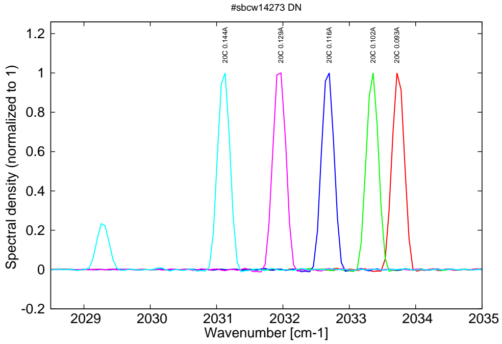
Figure 14: spectra at 20C for various DC currents (monomode up to 0.13A, then becomes bimode)
