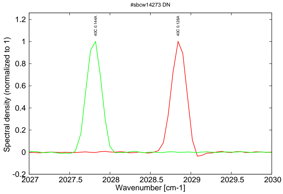
Figure 18: spectra at 40C for various DC currents (all monomode)
