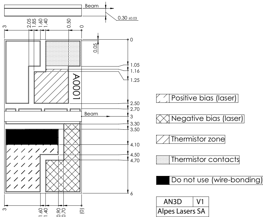
Figure 1: Mechanical and electrical interface for #sbcw14421 DN (please note that AlN submount numbering is P0349)
