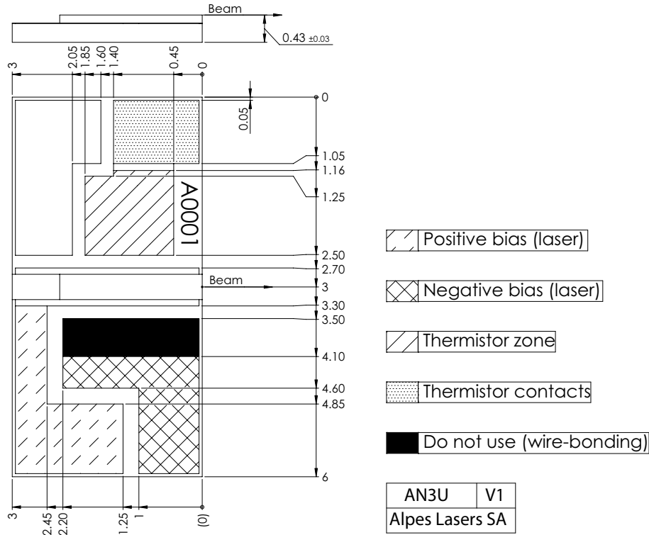
Figure 1: Mechanical and electrical interface for #sbcw15265 DN (please note that AlN submount numbering is A0CF6)
