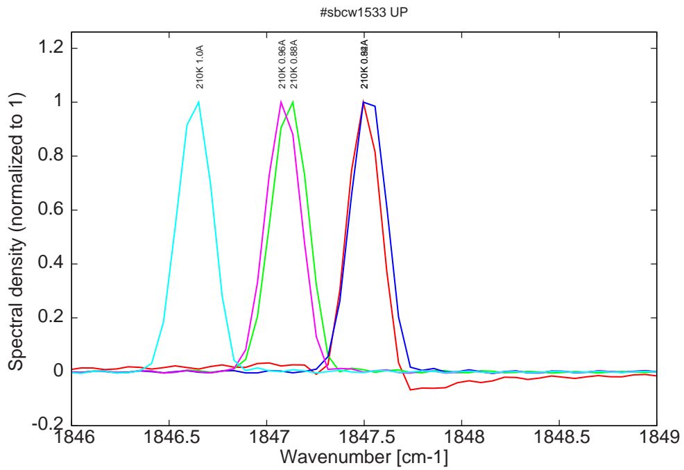
Figure 7: spectra at 210K for various DC currents (same mode as the other temperatures for I < 0.88A , mode jumping for I > 0.88A , see Fig. 1)
