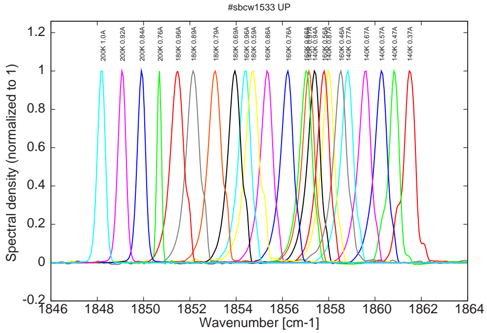
Figure 6: spectra at 140K, 160K, 180K and 200K for various DC currents
