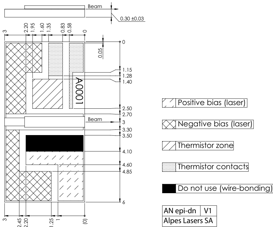
Figure 1: Mechanical and electrical interface for #sbcw15390 DN (please note that AlN submount numbering is A0065)
