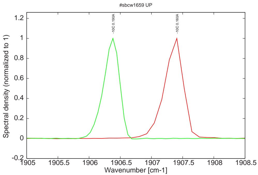
Figure 11: monomode spectra at -10C for various DC currents
