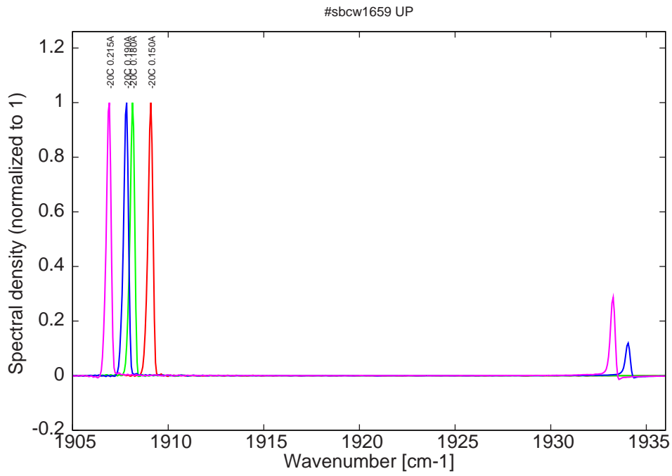
Figure 8: spectra at -20C for various DC currents (monomode up to 0.18A)
