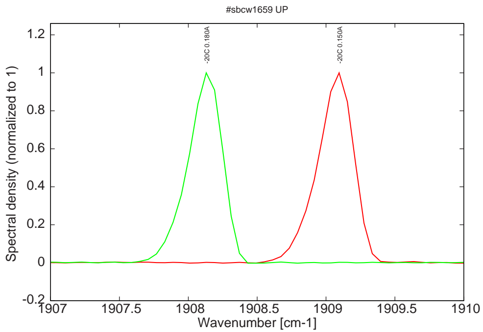
Figure 9: monomode spectra at -20C for various DC currents
