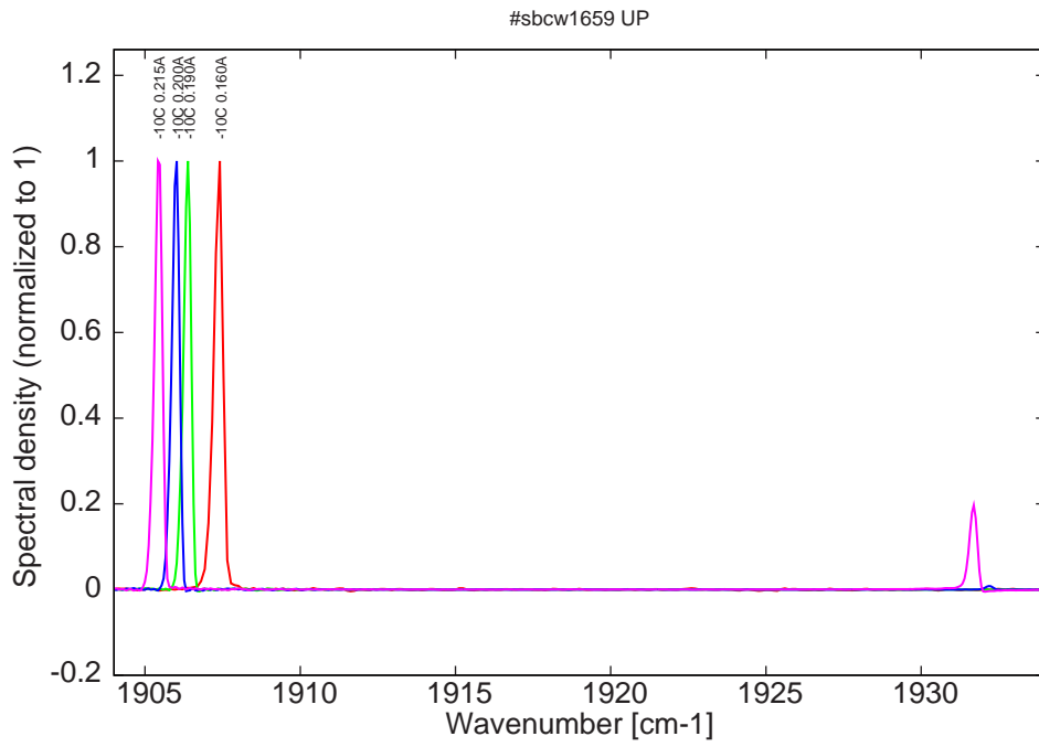
Figure 10: spectra at -10C for various DC currents (monomode up to 0.19A)
