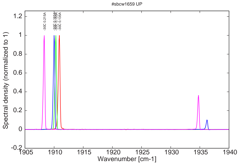
Figure 6: spectra at -30C for various DC currents (monomode up to 0.155A)
