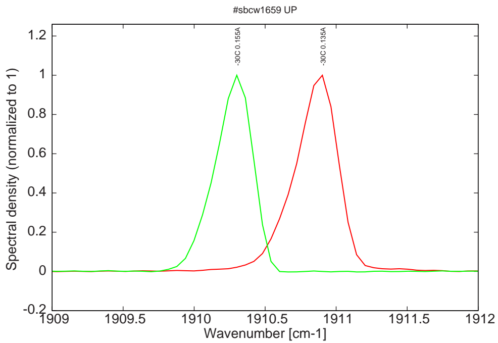
Figure 7: monomode spectra at -30C for various DC currents
