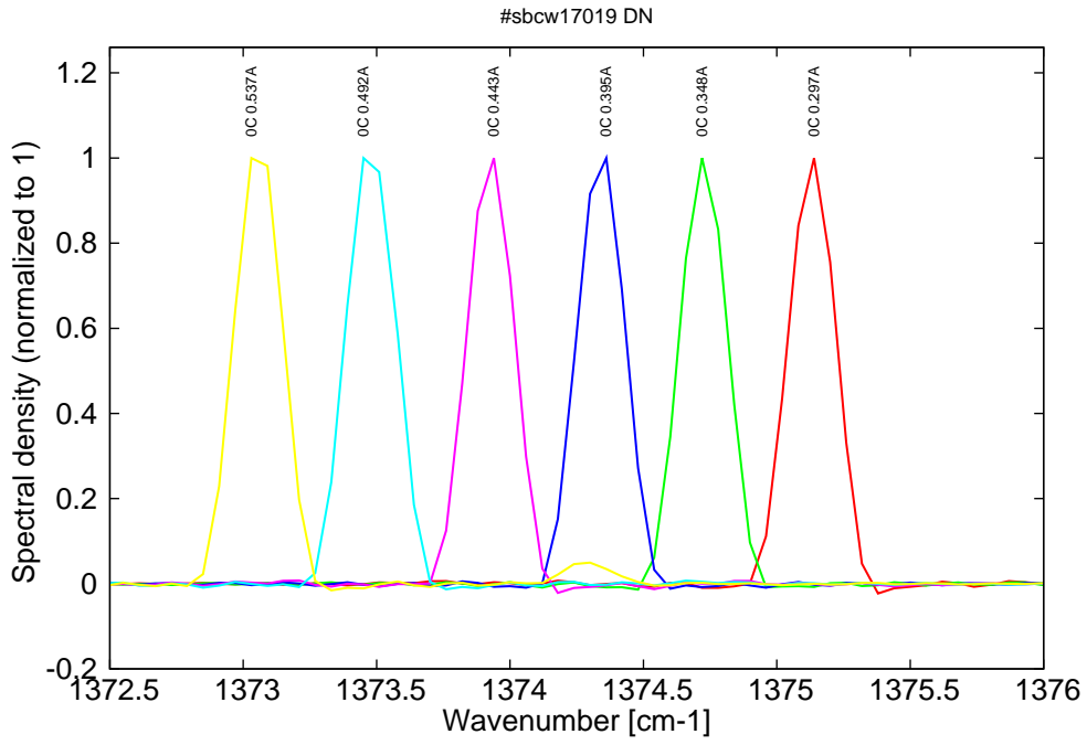
Figure 10: spectra at 0C for various DC currents (monomode up to 0.49A, then becomes bimode)
