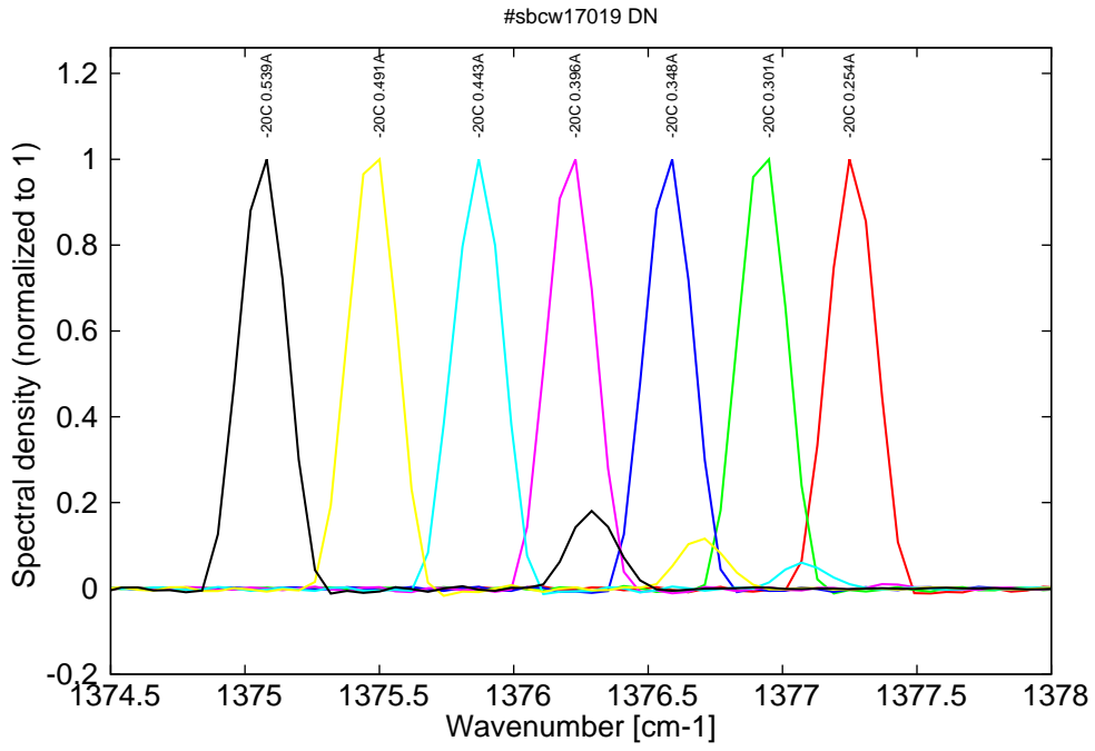
Figure 6: spectra at -20C for various DC currents (monomode up to 0.395A, then becomes bimode)
