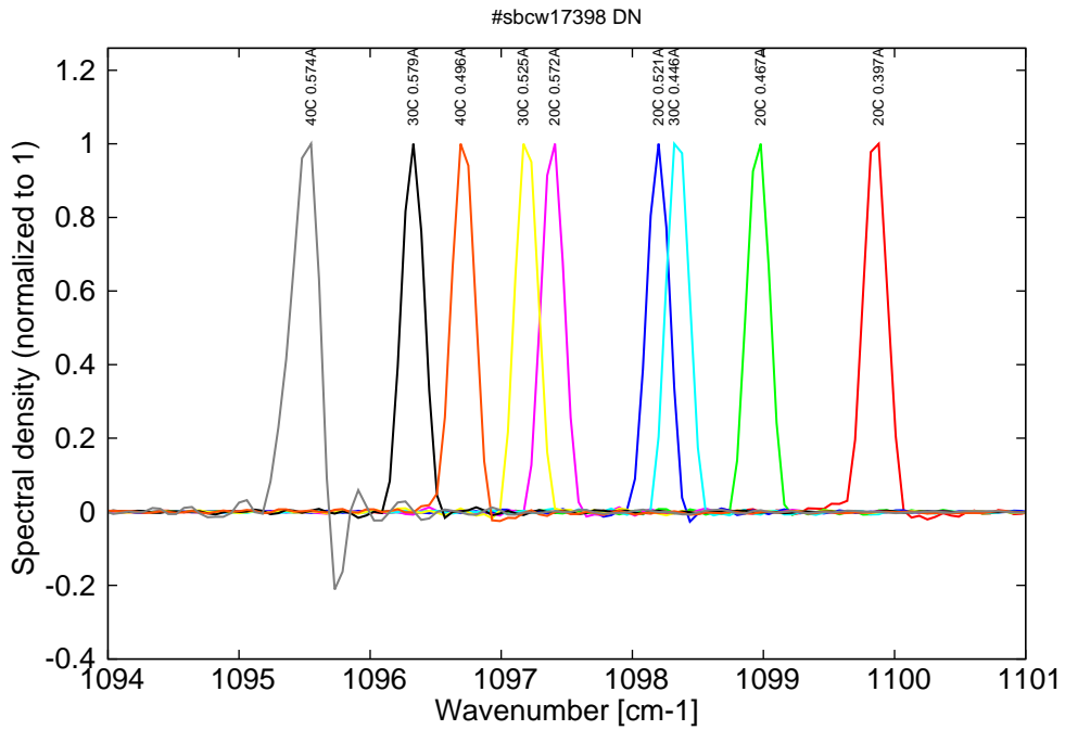
Figure 9: spectra between 20C and 40C for various DC currents (all monomode on mode 2)
