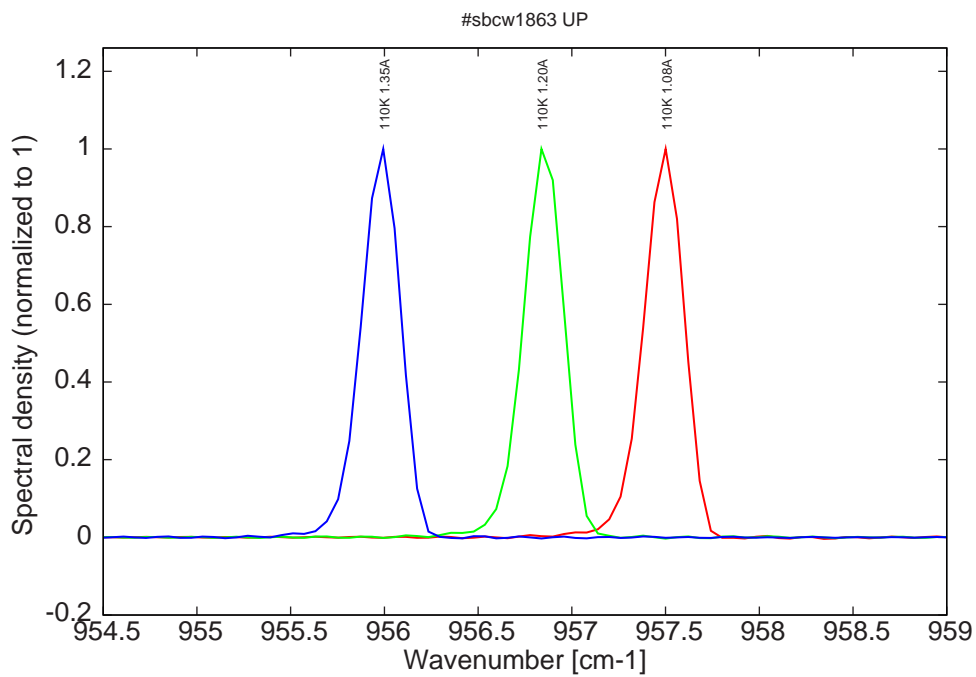
Figure 9: spectra at 110K for various DC currents (all monomode but on another mode, see Fig. 1)
