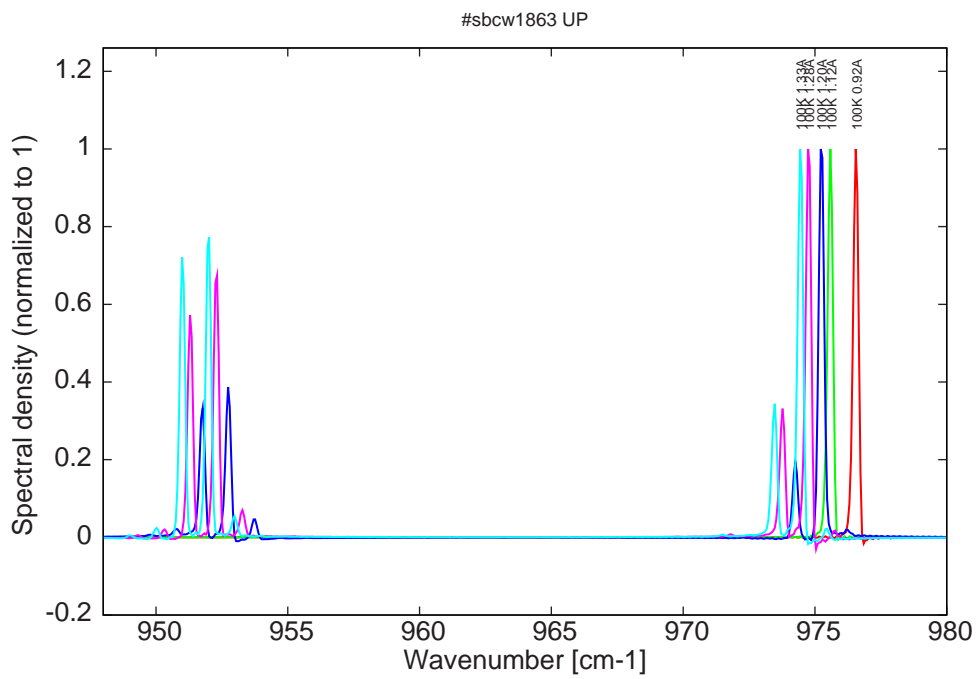
Figure 7: spectra at 100K for various DC currents (become multimode for I > 1.12A )
