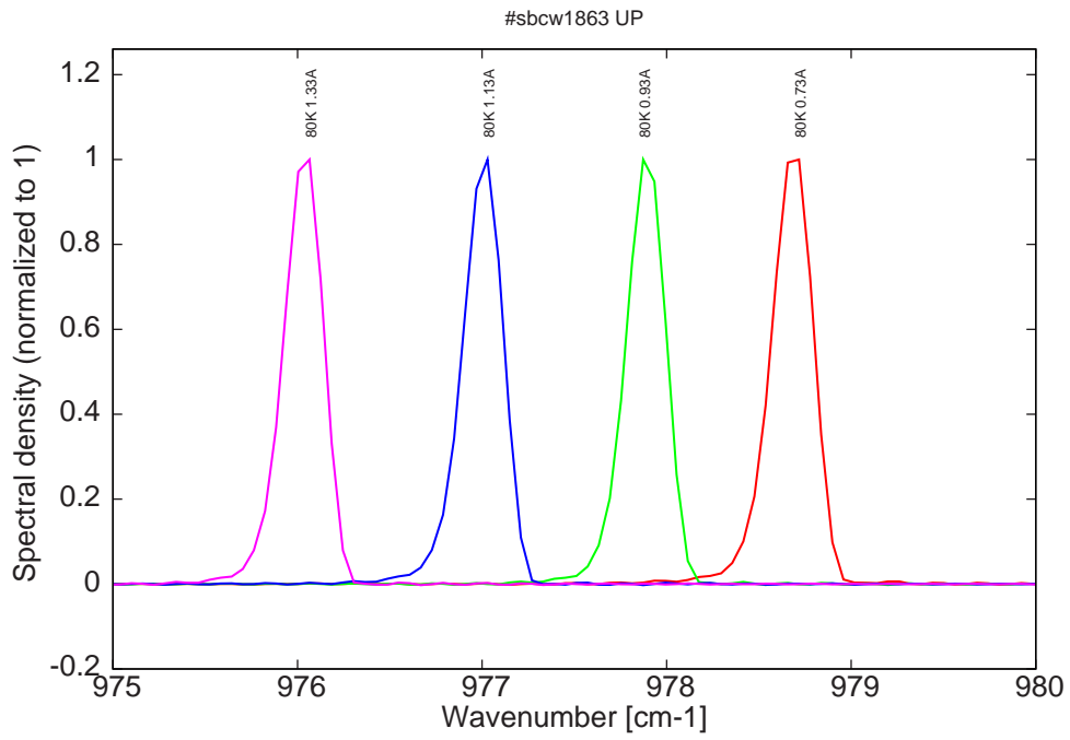
Figure 6: spectra at 80K for various DC currents (all monomode)
