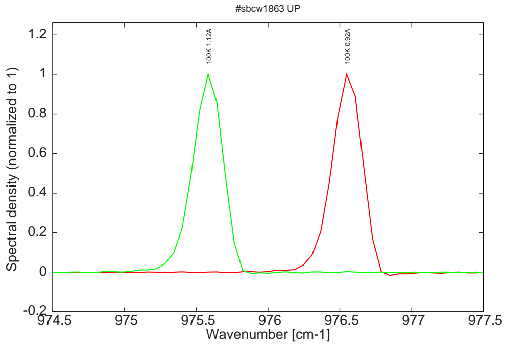
Figure 8: spectra at 100K for various DC currents (monomode range)
