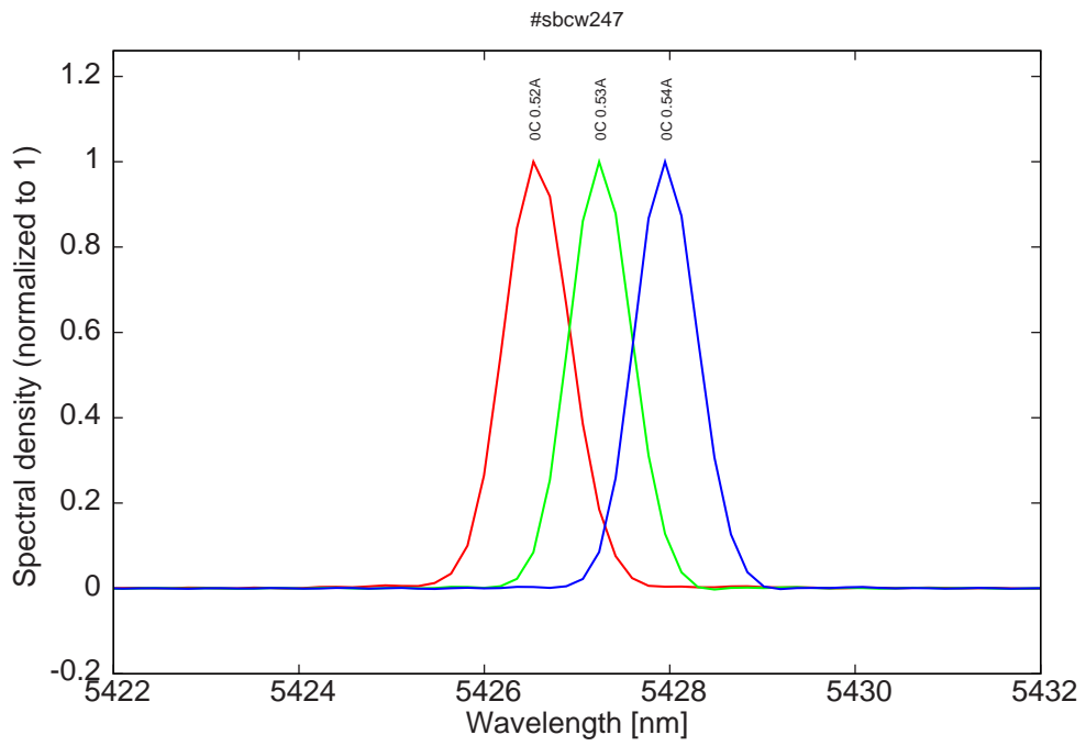
Figure 10: spectra at 0C for various DC currents
