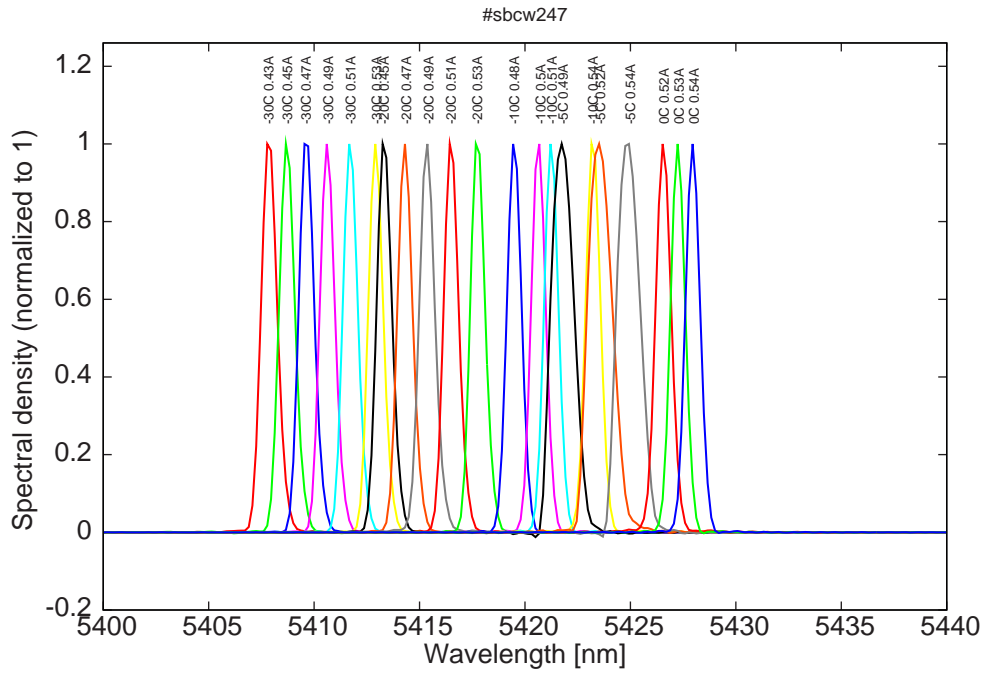
Figure 5: spectra at -30C, -20C, -10C, -5C and 0C for various DC currents
