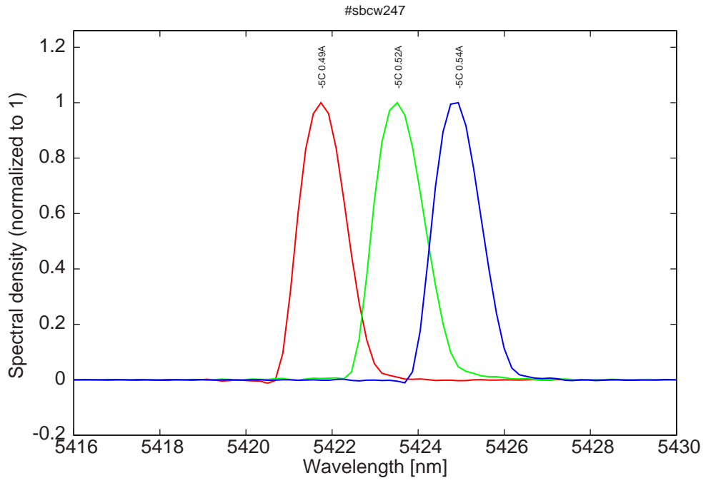
Figure 9: spectra at -5C for various DC currents
