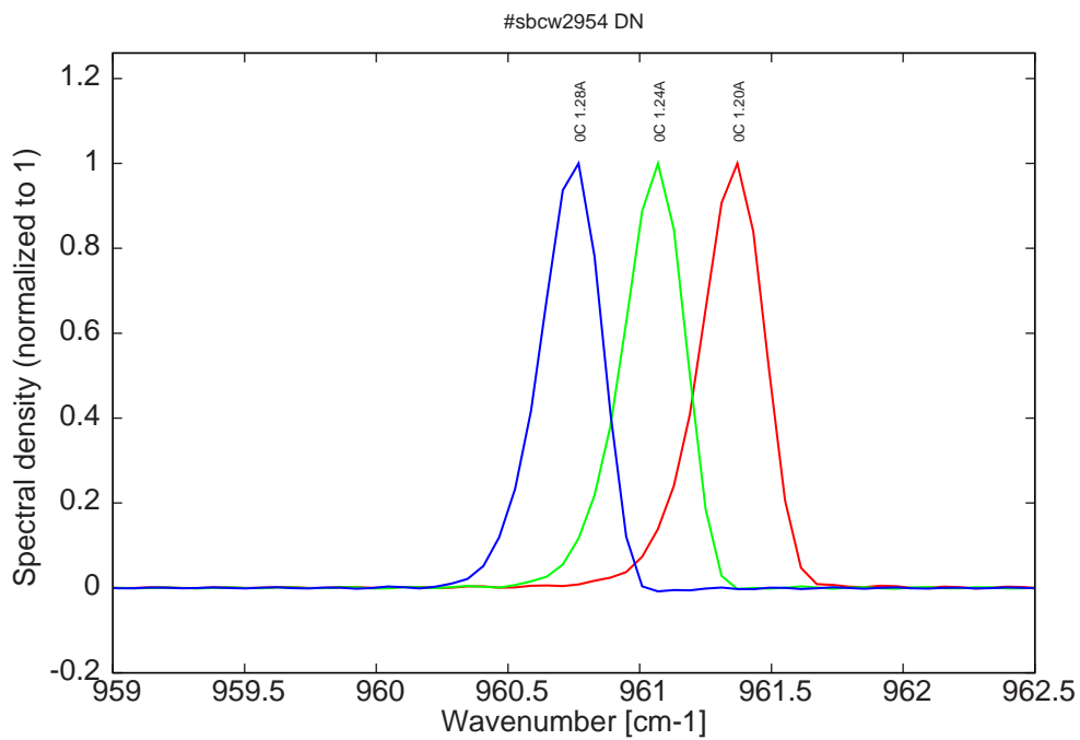
Figure 8: spectra at 0C for various DC currents (all monomode on the same mode, see Fig. 3)
