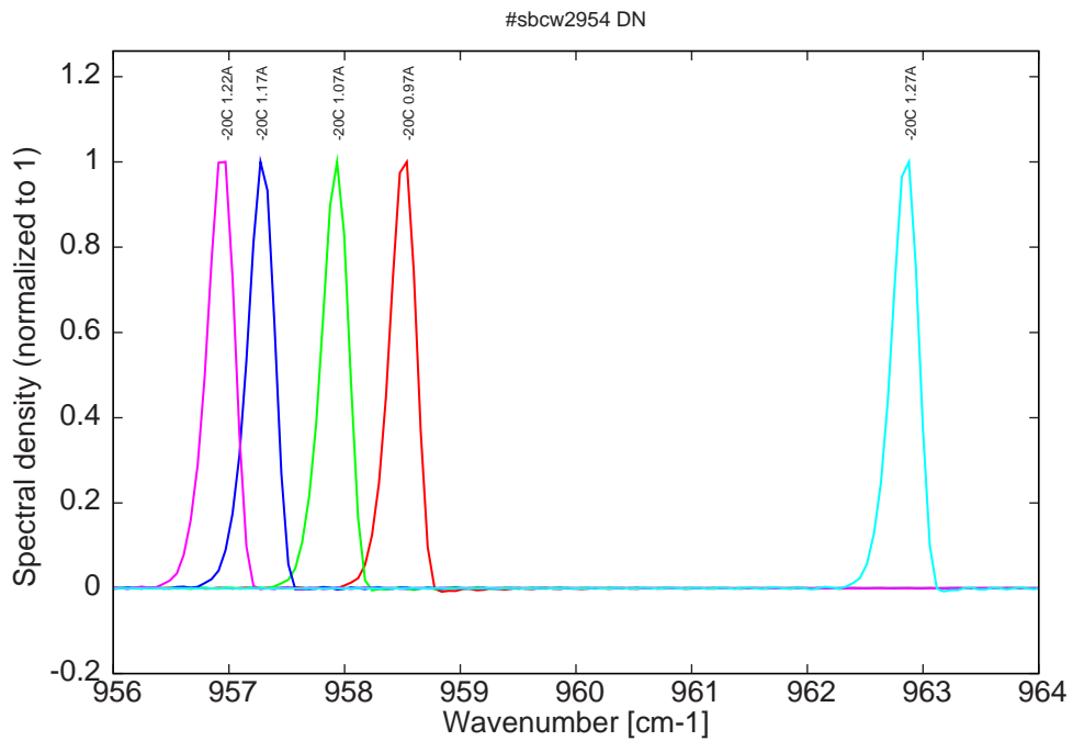
Figure 6: spectra at -20C for various DC currents (monomode with mode jumping for I > 1.22A , see Fig. 3)
