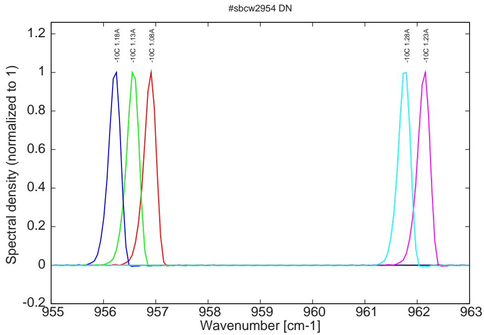
Figure 7: spectra at -10C for various DC currents (monomode with mode jumping for I > 1.18A , see Fig. 3)
