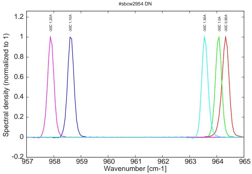
Figure 5: spectra at -30C for various DC currents (monomode with a first mode jumping for I > 1.0A and a second mode jumping for I > 1.2A , see Fig. 3)
