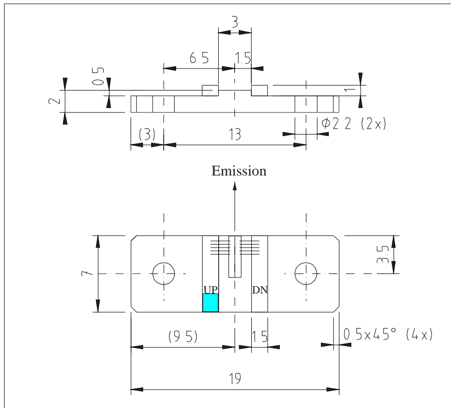
Figure 1: Support mounting for #sbcw3124 UP (please note that the laser is connected to the UP pad drawn in blue)
