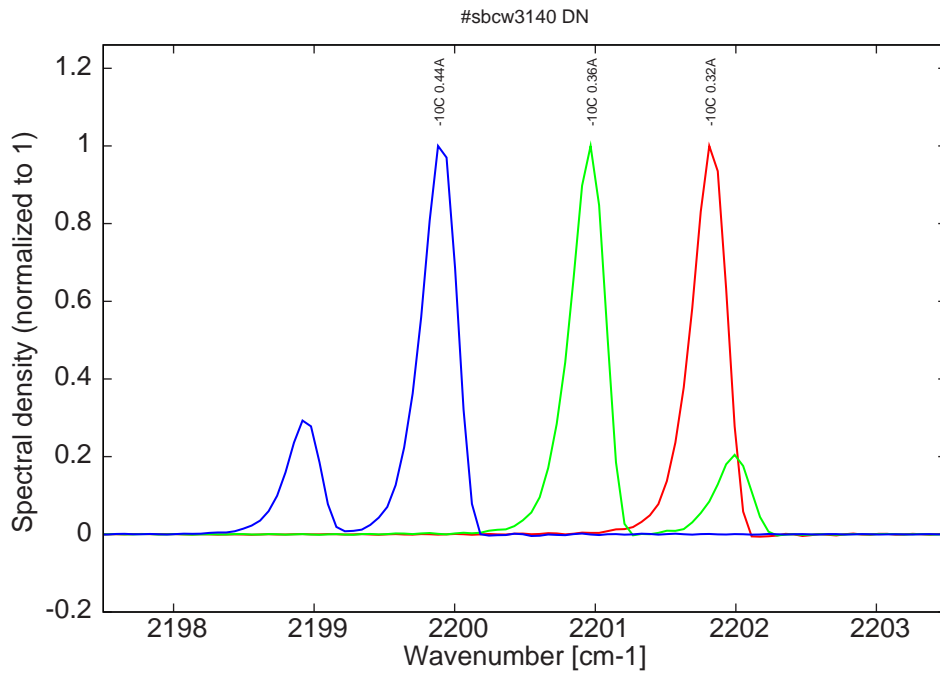
Figure 8: spectra at -10C for various DC currents (monomode on mode 1 only at threshold)
