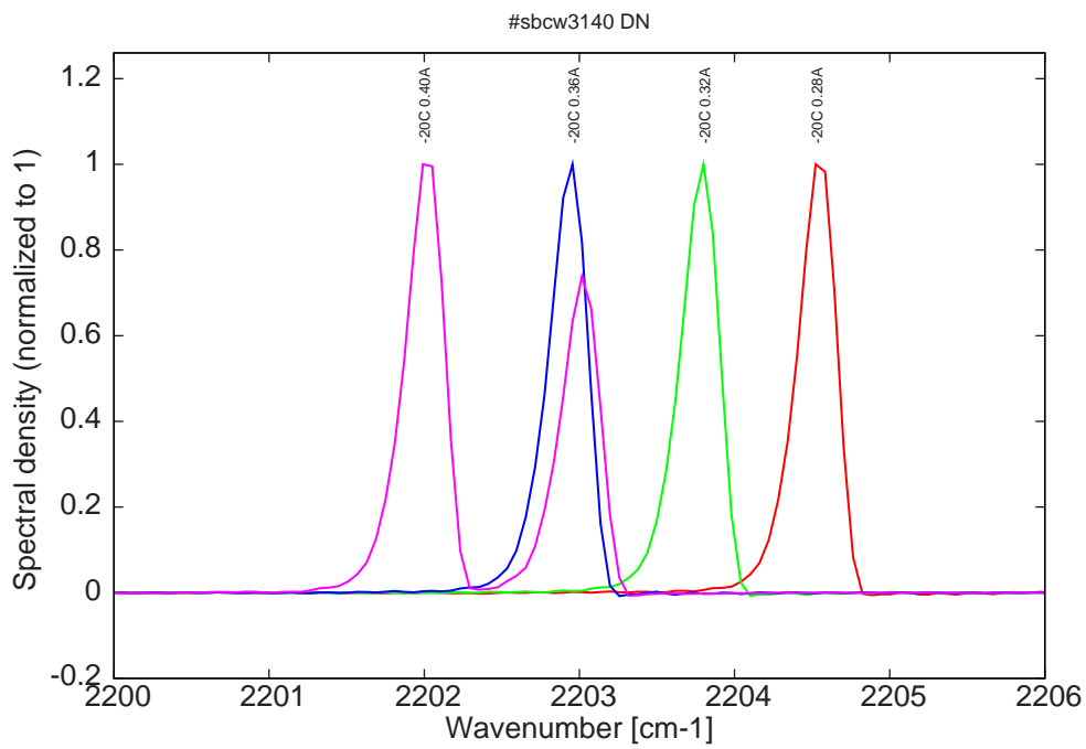
Figure 7: spectra at -20C for various DC currents (monomode on mode 1 up to 0.36A)
