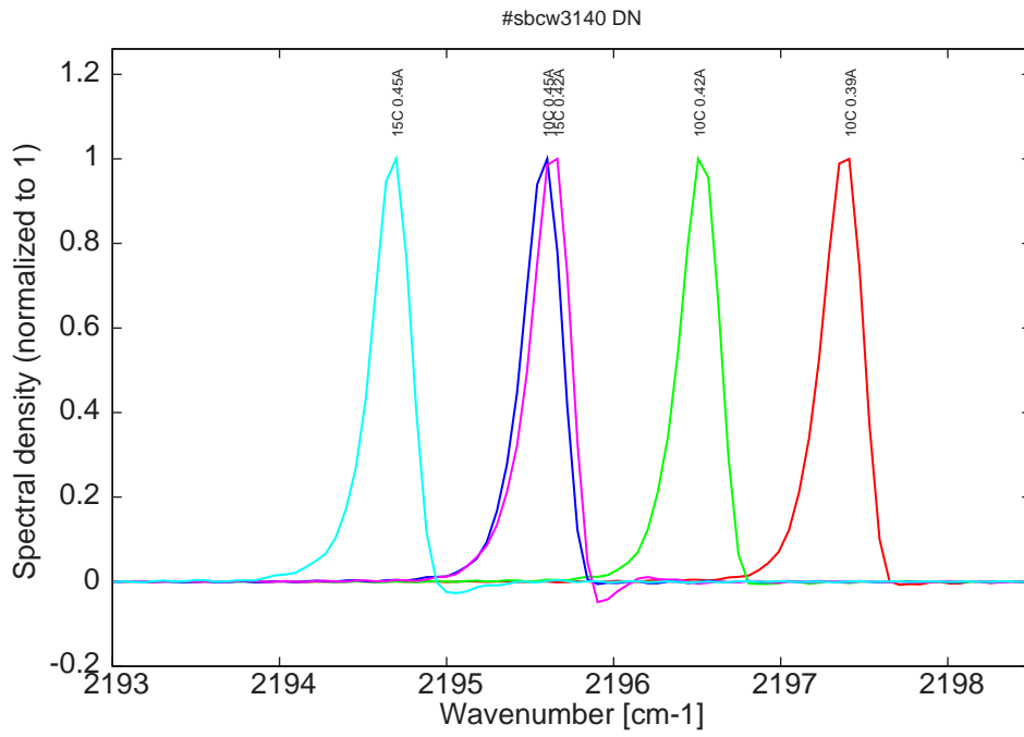
Figure 10: spectra between 10C and 15C for various DC currents (all monomode on mode 2, see Fig. 2 & 3)
