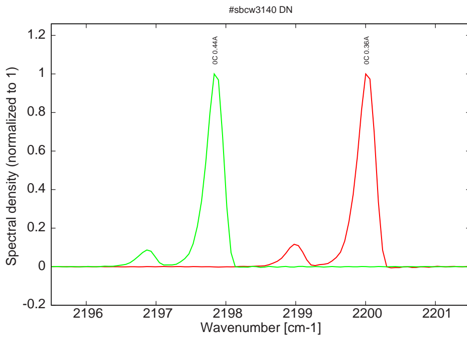
Figure 9: spectra at 0C for various DC currents (all bimode)
