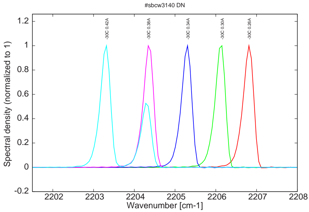
Figure 6: spectra at -30C for various DC currents (monomode on mode 1 up to 0.38A)
