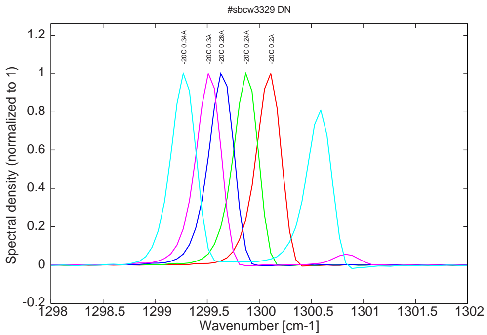
Figure 7: spectra at -20C for various DC currents (monomode up to 0.28A)
