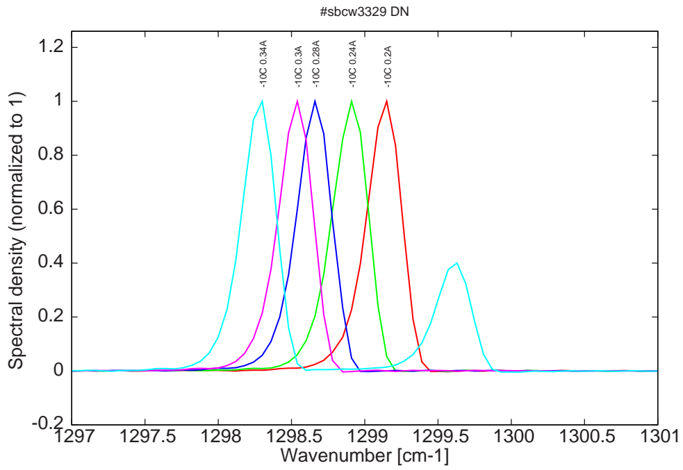
Figure 8: spectra at -10C for various DC currents (monomode up to 0.30A)
