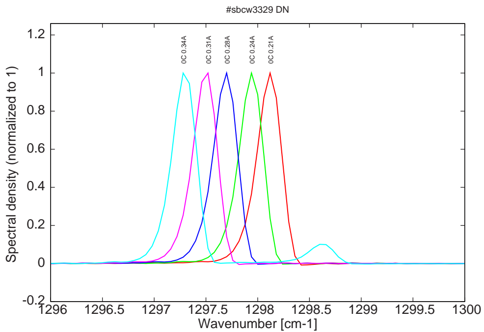
Figure 9: spectra at 0C for various DC currents (monomode up to 0.31A)
