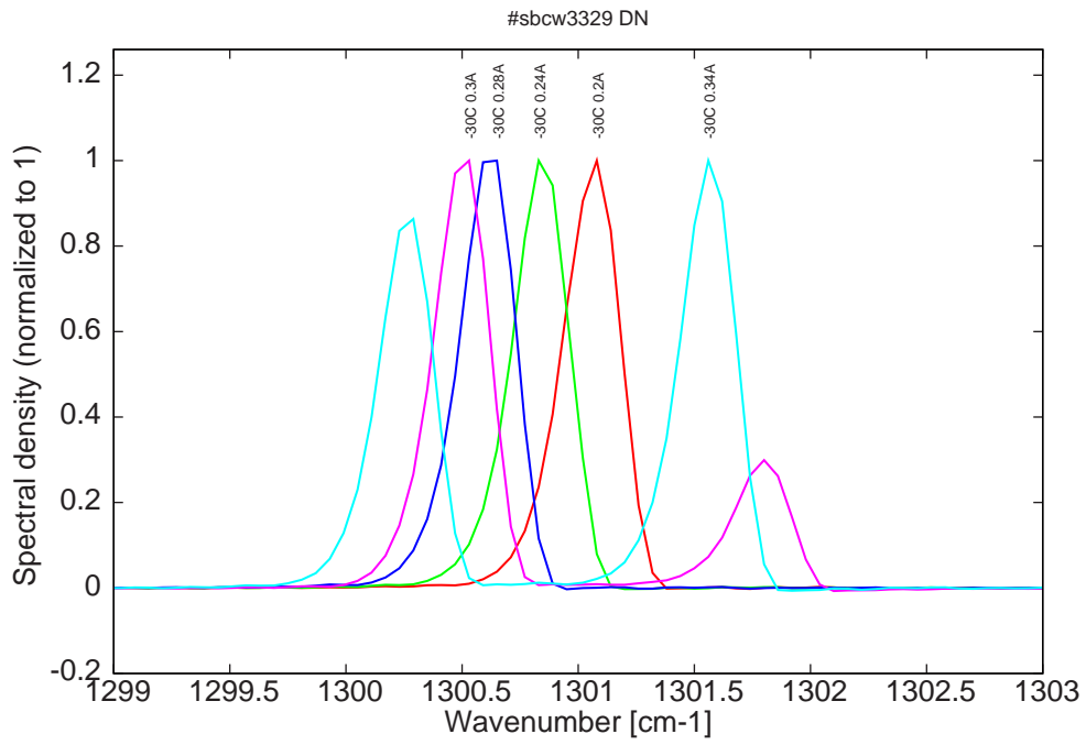
Figure 6: spectra at -30C for various DC currents (monomode up to 0.28A)
