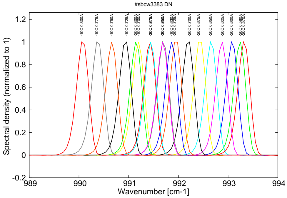
Figure 5: spectra at -20C and -10C for various DC currents (all monomode on mode 1, see Fig. 2 & 3)
