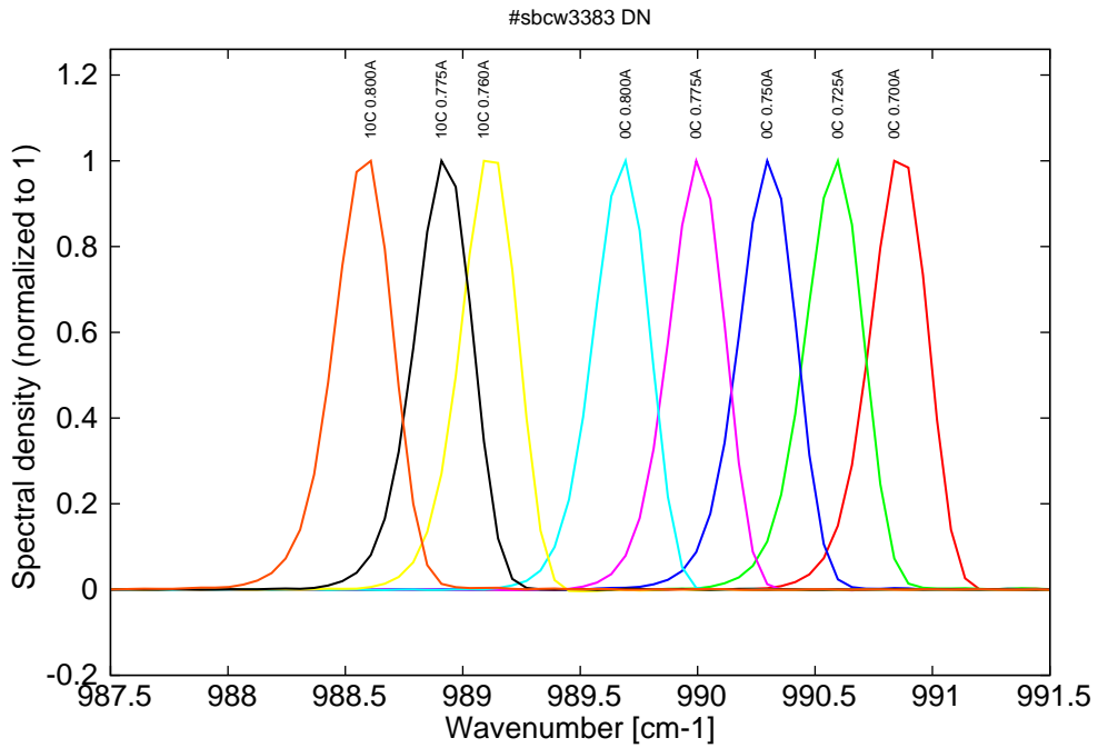
Figure 6: spectra at 0C and 10C for various DC currents (all monomode on mode 2, see Fig. 2 & 3)
