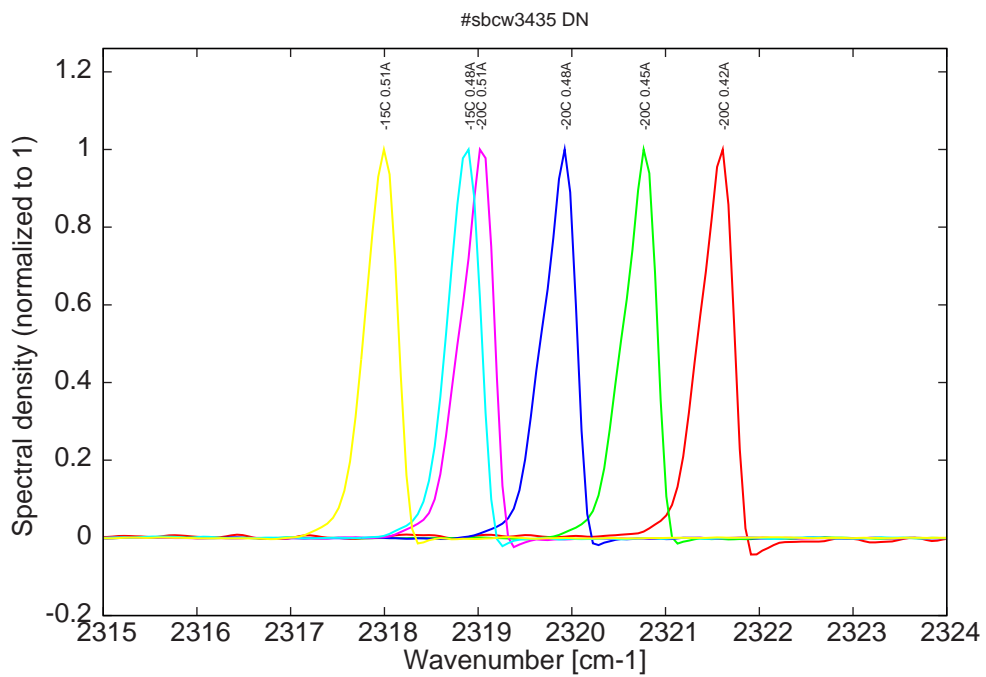
Figure 6: spectra at -20C and -15C for various DC currents (monomode on mode 2, see Fig. 2 & 3)
