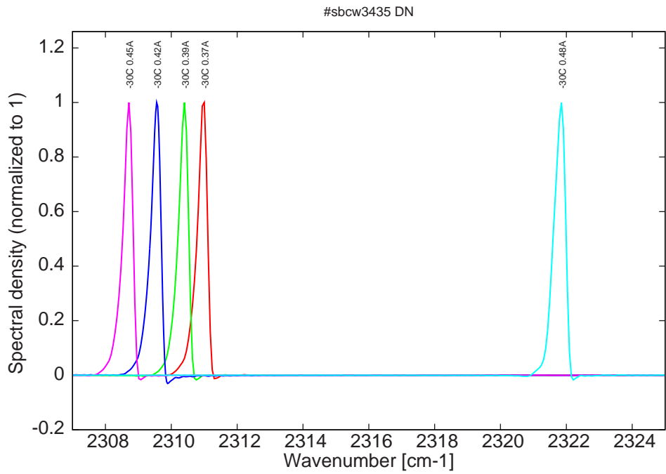
Figure 5: spectra at -30C for various DC currents (mode jumping for I > 0.45A , see Fig. 2 & 3; on mode 1 & 2)
